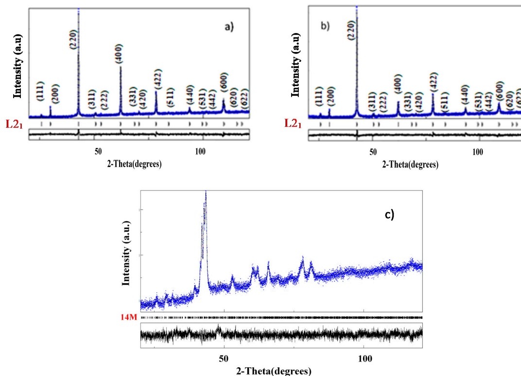
Figure 1. X-ray diffraction (XRD) diffractograms at room temperature: (a) Ni 49 Mn 36 Sn 14 Pd 1 , (b) Ni 48 Mn 36 Sn 14 Pd 2 , and (c) Ni 50 Mn 36 Sn 13 Pd 1 .
