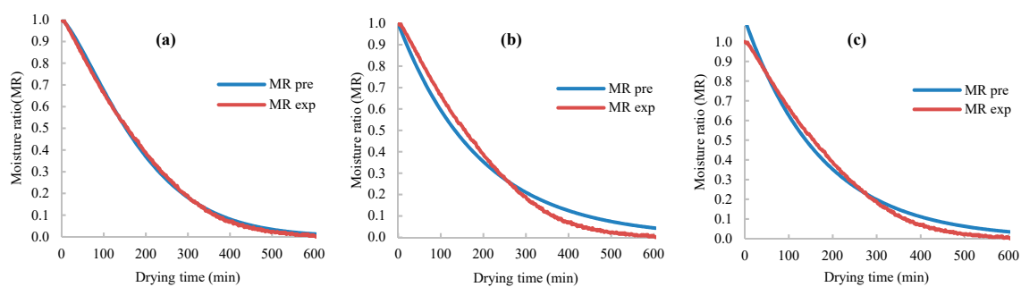
Figure 7. Comparison of experimental and calculated MR (45 °C, 0.20 m/s 6 mm): (a)-Page model, (b)-Newton (Lewis) model and (c)-Henderson and Pabis model.
