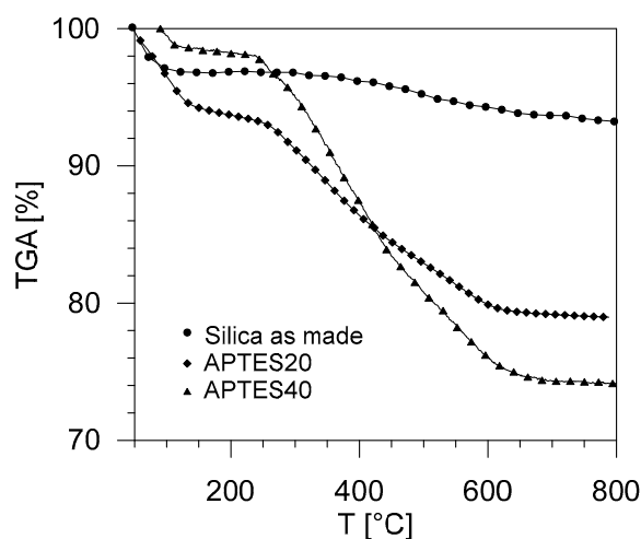
Figure 8. TGA analysis for the as-made silica, APTES20 and APTES40.
