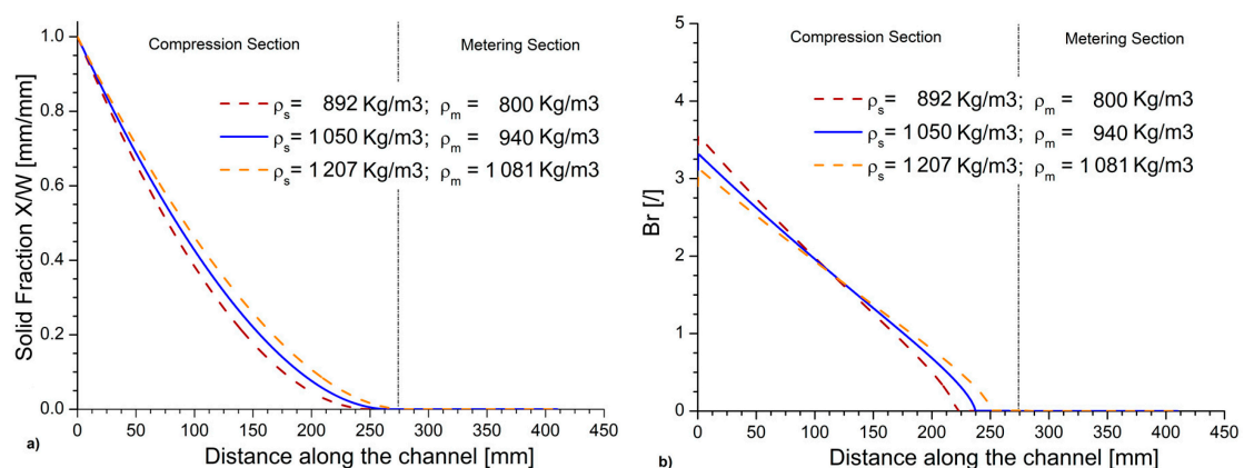
Figure 11. (a) Melting profile; and (b) Brinkman number for different polymer solid densities considering otherwise the micro-extrusion settings and material parameters of Table 1 (Column 2). Blue (reference) lines as in Figure 4.
