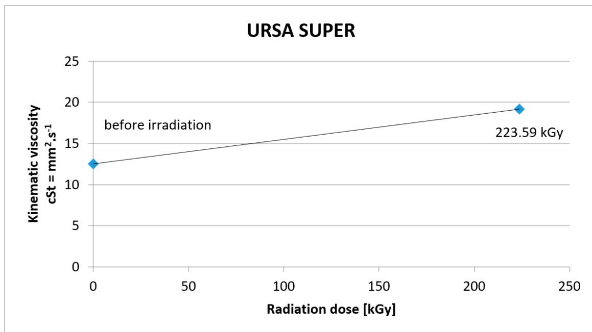
Figure 4. Increase of kinematic viscosity at high dose of irradiation.
