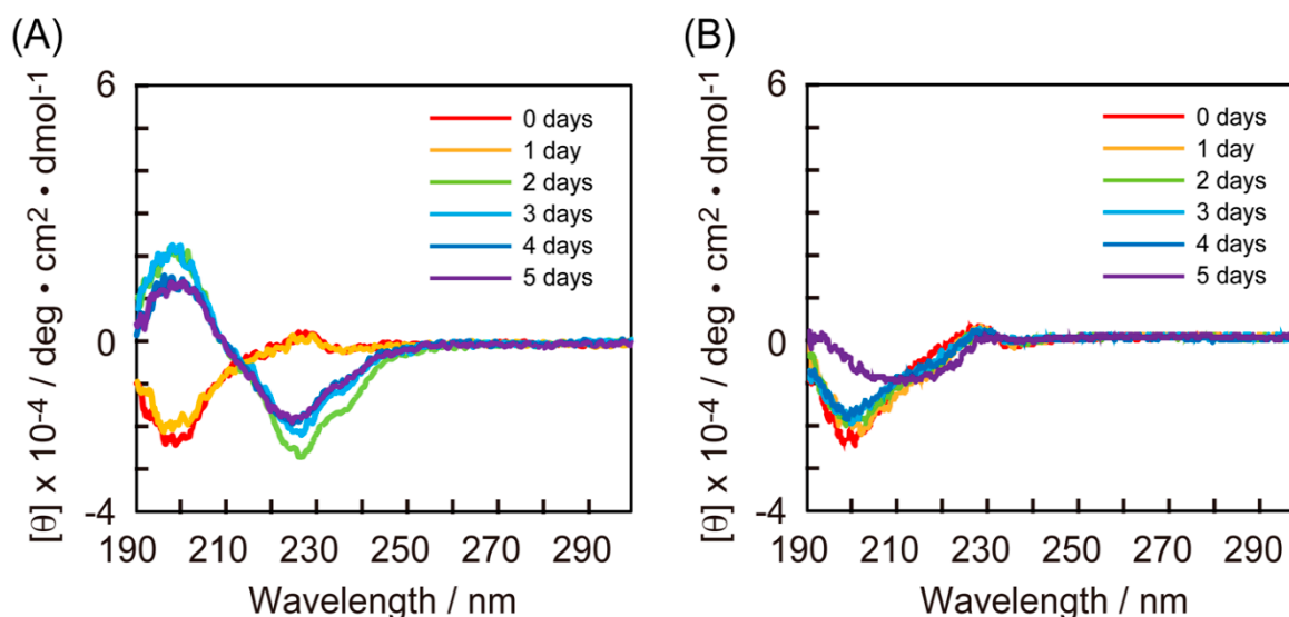
Figure 2. Typical circular dichroism (CD) spectra of RU003 in the (A) absence and (B) presence of Ape5-TD (conditions: [RU003] = 100 \mu M and [Ape5-TD] = 10 \mu M in water at 40 °C). The y -axis indicates the mean residue ellipticity. Incubation period “0 day” means “5 min after the reaction started”.
