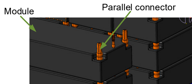
Figure 9. Example of parallel connection.
