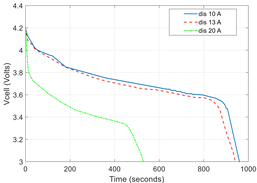
Figure 6. Cell discharge results.
