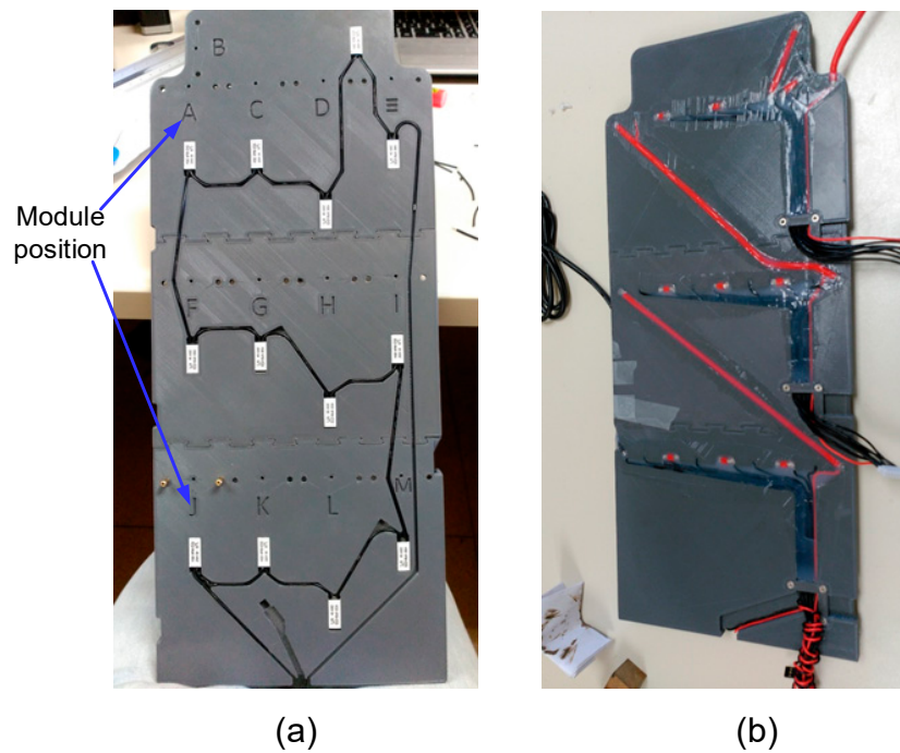
Figure 7. Current collector codification (a) and connections (b).
