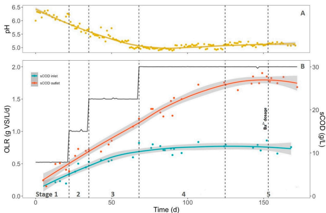
Figure 2. Organic loading rate (OLR) along the operation of the anaerobic semi-continuous hydrolytic reactor (ASHR) and monitoring results. (A—pH results, B—OLR and soluble chemical oxygen demand (sCOD) results). The grey areas represent the confidence interval of the non-linear regression line.
