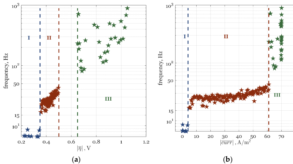
Figure A2. Optimal frequencies of modulation at different time-average: (a) overpotentials (CI) and (b) current densities (BI). The optimal solutions are displayed in the three distinct Zones: Zone I, of dominant kinetics and no ORR (blue stars); Zone II, where the FP operation is superior (red stars); and Zone III, where the FP operation offers a negligible PI potential (green stars).
