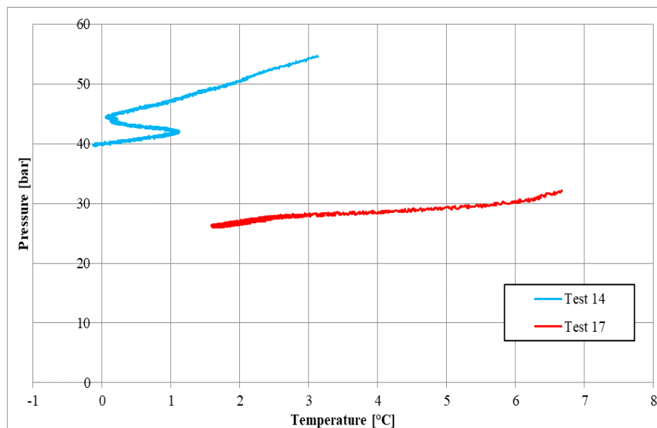
Figure 11. Comparison between Test 14, carried out using \text{CH}_4 , and Test 17, performed with \text{CO}_2 .
