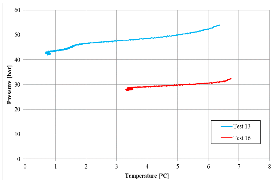
Figure 10. Comparison between Test 13, carried out using \text{CH}_4 , and Test 16, performed with \text{CO}_2 .
