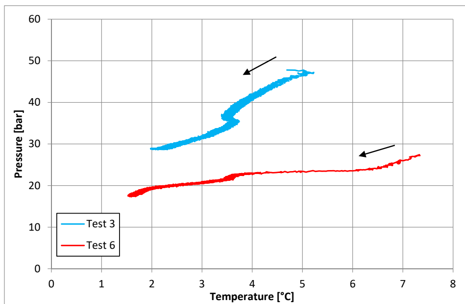
Figure 6. Comparison between Test 3, carried out using \text{CH}_4 , and Test 6, performed with \text{CO}_2 .
