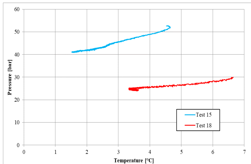
Figure 12. Comparison between Test 15, carried out using CH 4 , and Test 18, performed with CO 2 .
