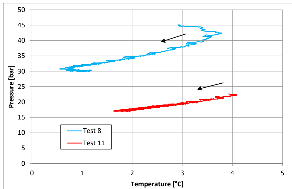
Figure 8. Comparison between Test 8, carried out using \text{CH}_4 , and Test 11, performed with \text{CO}_2 .
