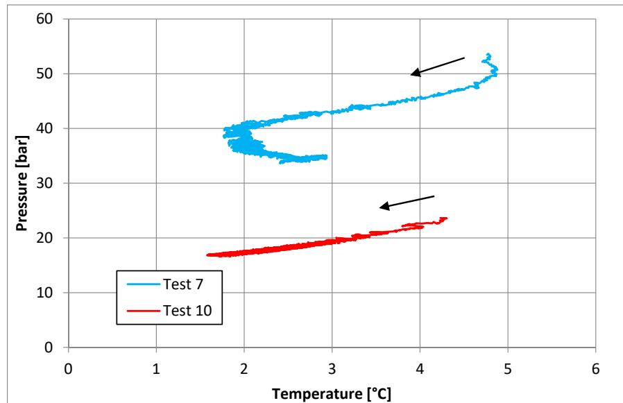
Figure 7. Comparison between Test 7, carried out using \text{CH}_4 , and Test 10, performed with \text{CO}_2 .
