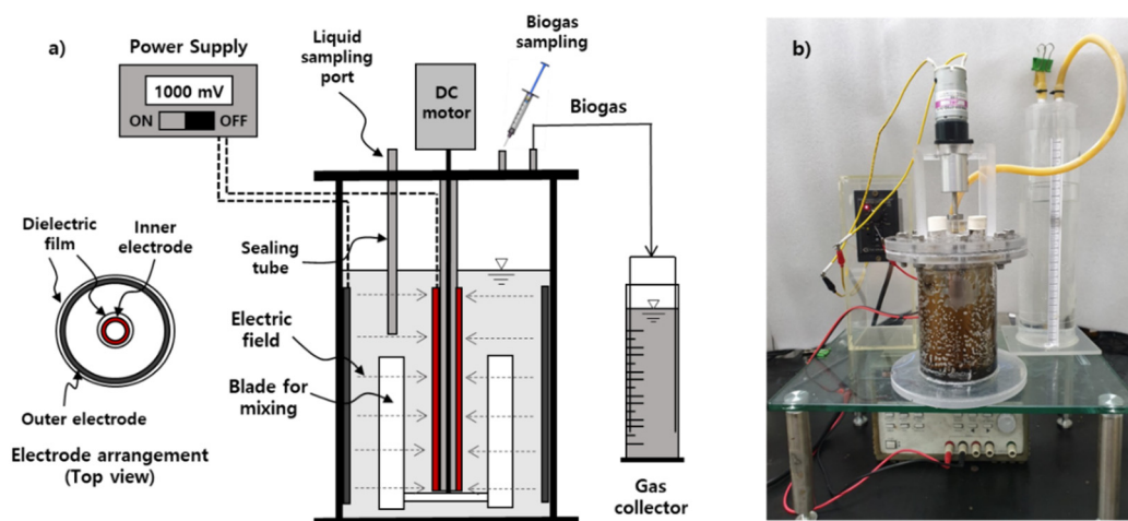
Figure 1. Bioelectrochemical anaerobic batch reactor used in the experiment: (a) schematic diagram, (b) photograph.
