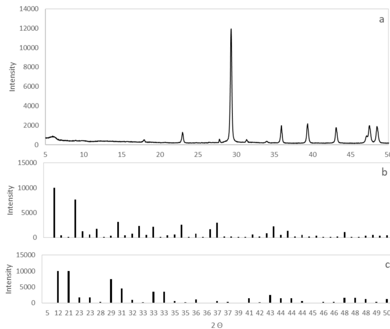
Figure 5. X-ray diffractogram of (a) S_40 sample compared with (b) a ettringite diffractogram and (c) a gypsum diffractogram from the database.
