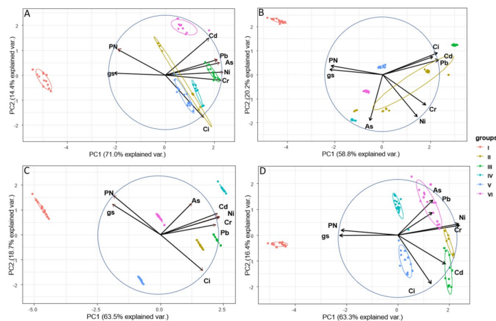
Figure 5. Principal component analysis of photosynthesis activity parameters and trace elements concentrations (arrows) and samples from each exposure sites (points) in four exposure series (A–D, respectively). Ellipses represent the confidence intervals of points.
