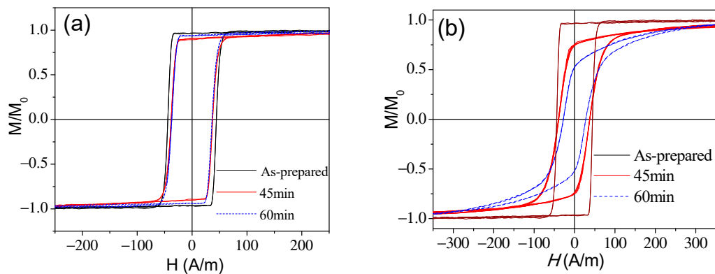
Figure 16. Hysteresis loops of as-prepared and annealed at T_{ann} = 325 °C (a) and as-prepared and stress-annealed at T_{ann} = 325 °C and \sigma_m = 190 MPa (b) \text{Fe}_{75}\text{B}_9\text{Si}_{12}\text{C}_4 microwire. Adapted from [98].
