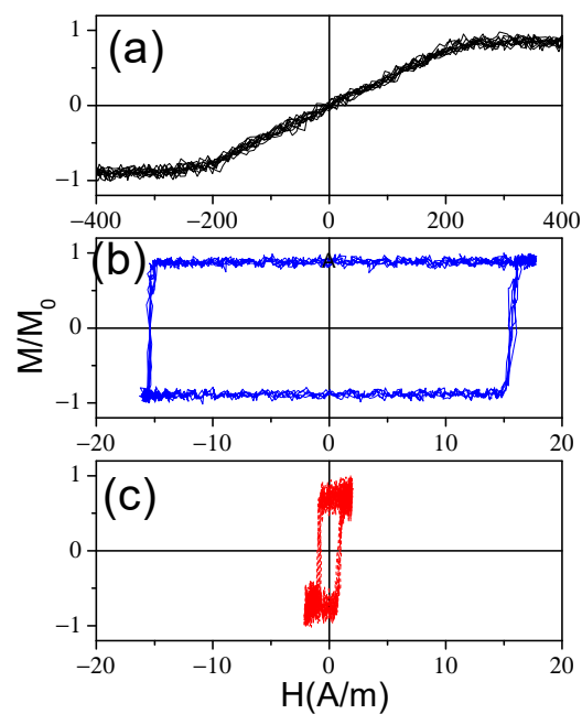
Figure 21. Hysteresis loops of as-prepared (a), annealed at T_{ann} = 350\text{ }^{\circ}\text{C} (b) and stress annealed at T_{ann} = 350\text{ }^{\circ}\text{C} and \sigma_m = 250\text{ MPa} (c) \text{Co}_{68.7}\text{Fe}_4\text{Ni}_1\text{B}_{13}\text{Si}_{11}\text{Mo}_{2.3} microwires. Adapted from Ref. [102].
