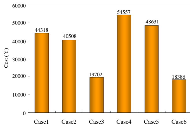
Figure 13. Operation and maintenance costs of island microgrid without rigid load compensation.
