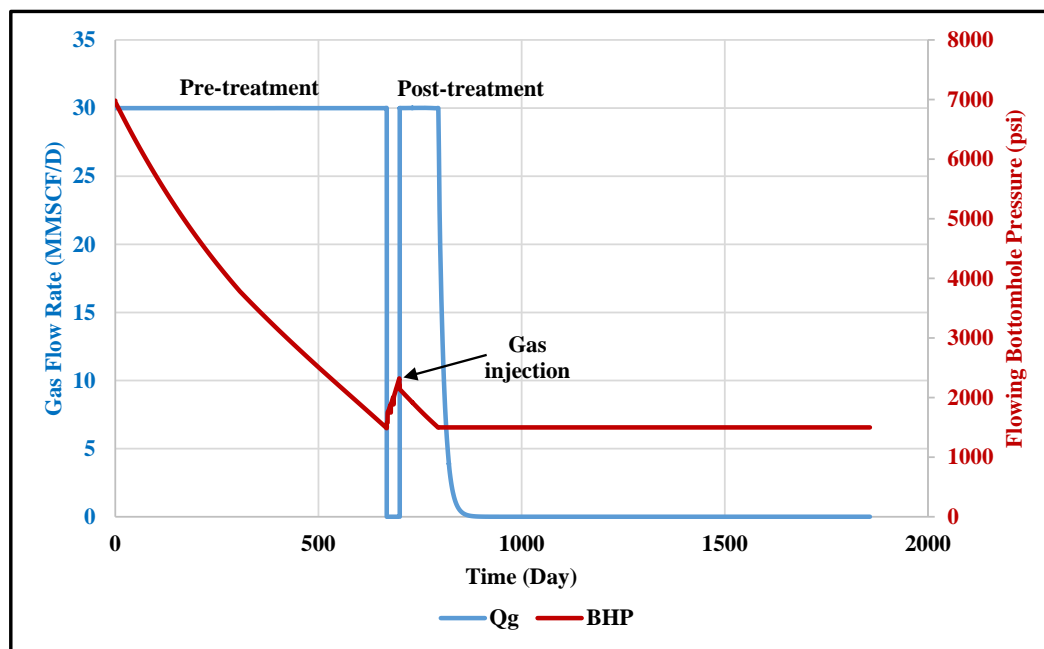
Figure 20. Profiles of gas production and associated flowing bottom-hole pressure before and after gas-injection treatment.
