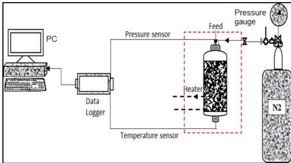
Figure 2. Experiment setup for monitoring thermochemical process.
