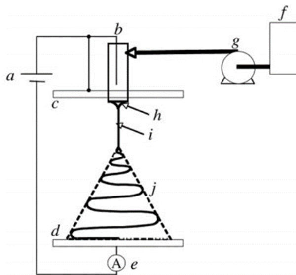
Figure 2. Schematic illustration of an experimental set up of a conventional electrospinning process: (a) high-voltage supply, (b) charging device of the spinneret, (c) high-potential electrode, (d) grounded collector, (e) current measurement device, (f) working solution reservoir, (g) flow rate control of the syringe pump, (h) Taylor's cone, (i) thinning jet and (j) instability region. Reprinted with permission from [16].
