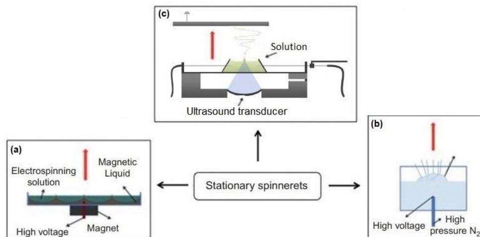
Figure 4. Schematic diagram depicting the stationary spinnerets: (a) ferromagnetic liquid, (b) bubble and (c) ultrasound-enhanced electrospinning, USES (electrospinning direction along the red arrow). Adapted with permission (CC BY 3.0) from [39,45].
