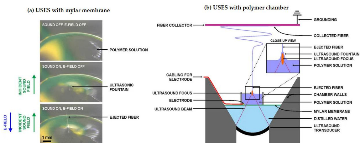
Figure 5. (a) An ultrasound-enhanced electrospinning (USES) method with a mylar membrane and (b) a USES system with a polymer chamber. Reprinted with permission (CC BY 3.0) from [26].
