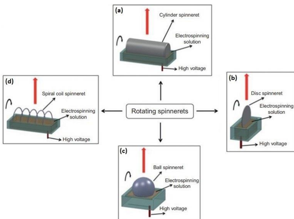
Figure 3. Schematic diagram depicting the rotating spinnerets: (a) cylinder spinneret, (b) disc spinneret, (c) ball spinneret and (d) wire/coil spinneret in needleless electrospinning (electrospinning direction along the red arrow). Adapted with permission (CC BY 3.0) from [39].
