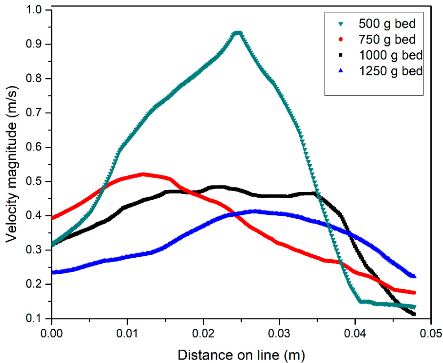
Figure 10. Comparison of average velocity profiles of different bed weights at 60^\circ .
