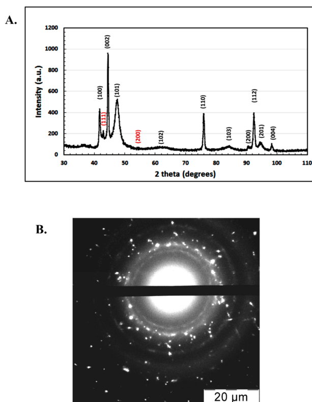
Figure 1. (A) X-ray diffraction ( \text{Cu K}\alpha ), and (B) selected area electron diffraction (SAED) results on synthesized Co nanopowders.
