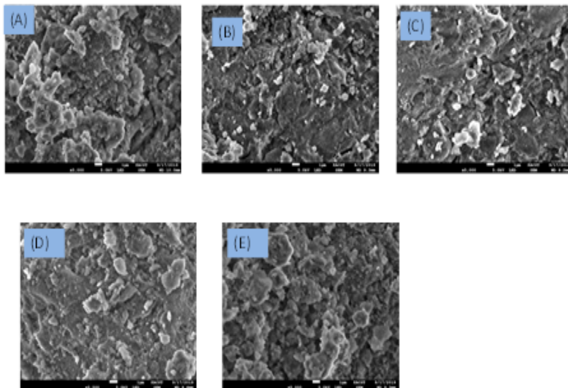
Figure 6. SEM images of the fresh catalysts (A) 5Ni/Al, (B) 5Ni+1Gd/Al, (C) 5Ni+1Zn/Al, (D) 5Ni+1Cu/Al, and (E) 5Ni+1Ga/Al.
