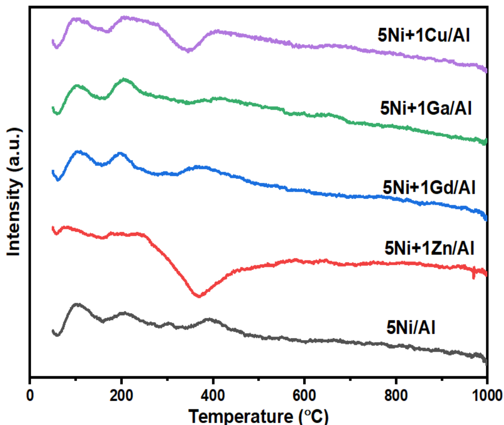
Figure 4. Temperature programmed oxidation (TPO) profiles of the used catalysts.
