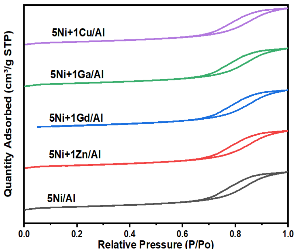
Figure 1. N 2 adsorption-desorption isotherms for non-promoted and promoted catalysts.
