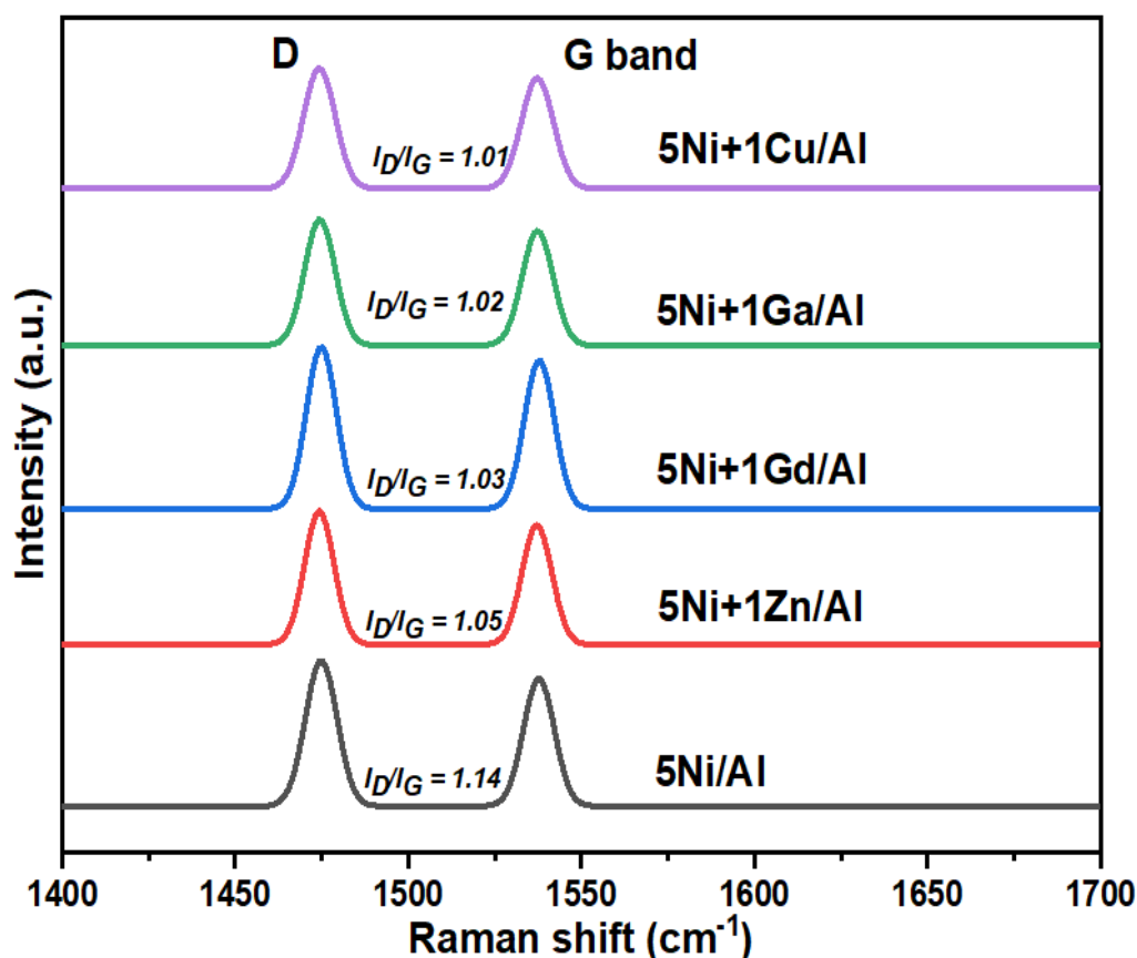
Figure 7. Raman spectra for the spent catalysts.
