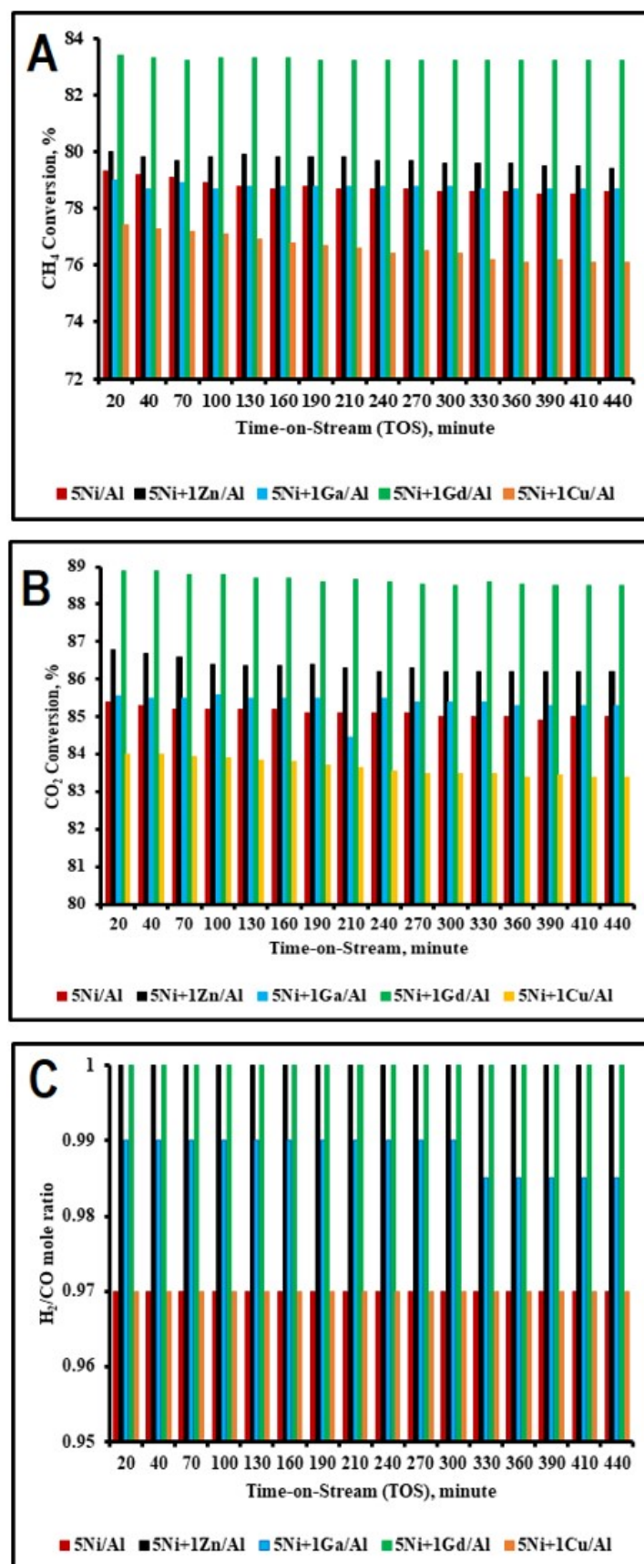
Figure 3. (A) Conversion of CH 4 , (B) Conversion of CO 2 , and (C) the fraction of H 2 /CO at 700 °C, 1.0 atm and GHSV = 2990 h -1 .
