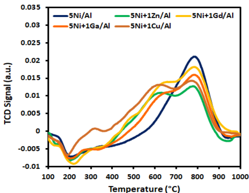
Figure 2. Temperature-programmed reduction (TPR) profiles of the non-promoted and promoted catalysts.
