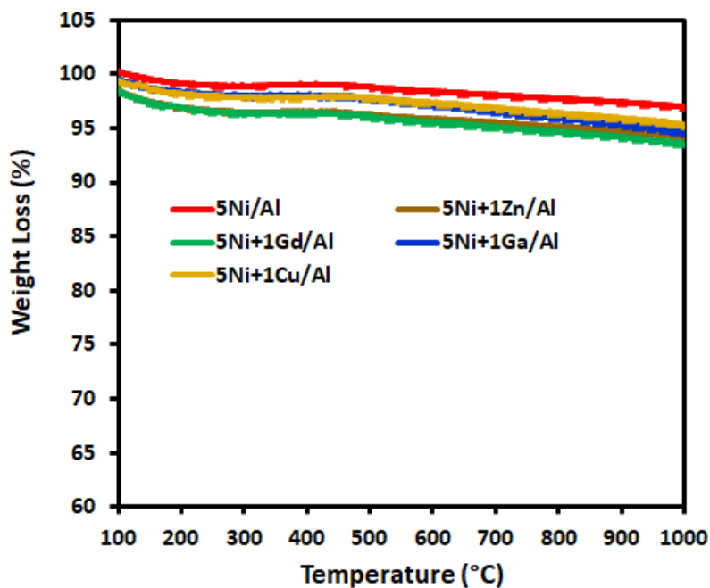
Figure 5. Thermogravimetric analysis (TGA) curves of the spent catalysts.
