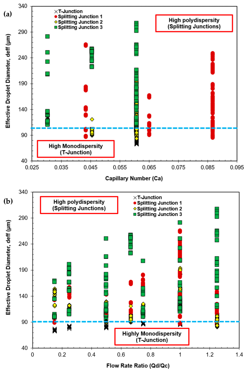
Figure 19. Distribution of droplet size in various regions of interest with respect to: (a) Capillary number and (b) Flow rate ratio at asymmetrical bifurcating junction.
