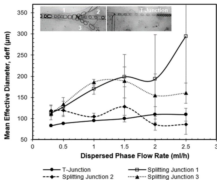
Figure 12. Average droplet size distribution with respect to different Q_d ranging from 0.3 to 2.5 mL/h in symmetrical bifurcating junction. Image indicates the region of interest for the droplet measurement. Error bars indicate the standard deviation in effective droplet size measurement of 30 droplets under fixed experimental condition.
