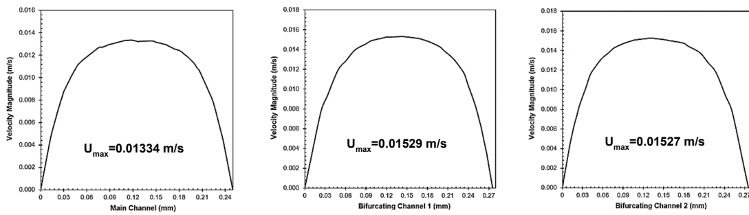
Figure 6. Evolution of flow profile at the upstream T-junction and downstream of symmetrical and asymmetrical splitting junctions (for system: Q_c = 2 mL/h).
