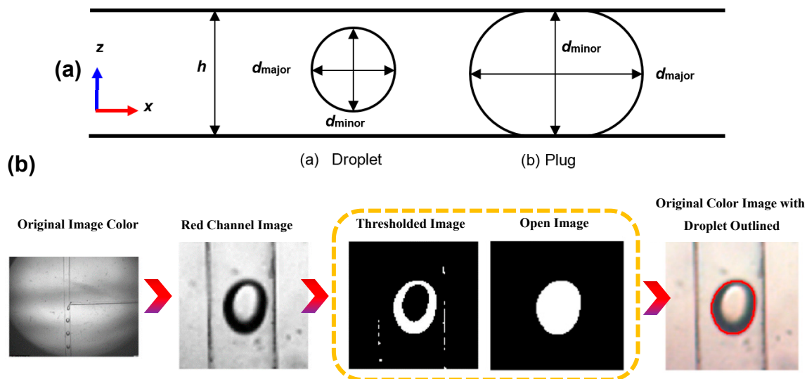
Figure 4. (a) Schematic diagram of the shape of confined droplets and plugs in microchannel. Major droplet diameter ( d_{\text{major}} ) denotes the longest dimension of the projected area of droplet/plug whereas the minor droplet diameter ( d_{\text{minor}} ) indicates the shortest dimension of the projected area of droplet/plug. The depth of the microchannel was denoted as h . (b) Image thresholding analysis of droplet or plug diameter in microchannel using MATLAB.
