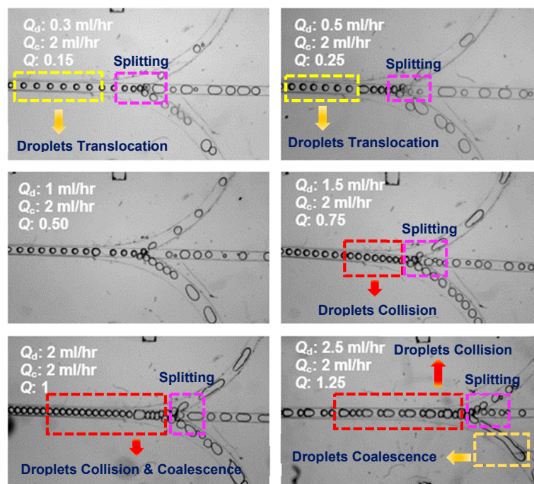
Figure 18. Droplet collision and coalescence phenomena in asymmetrical splitting junctions at different flow rate ratio ( 0.15 < Q < 1.25 ) by fixing the Q_c and varying the Q_d .
