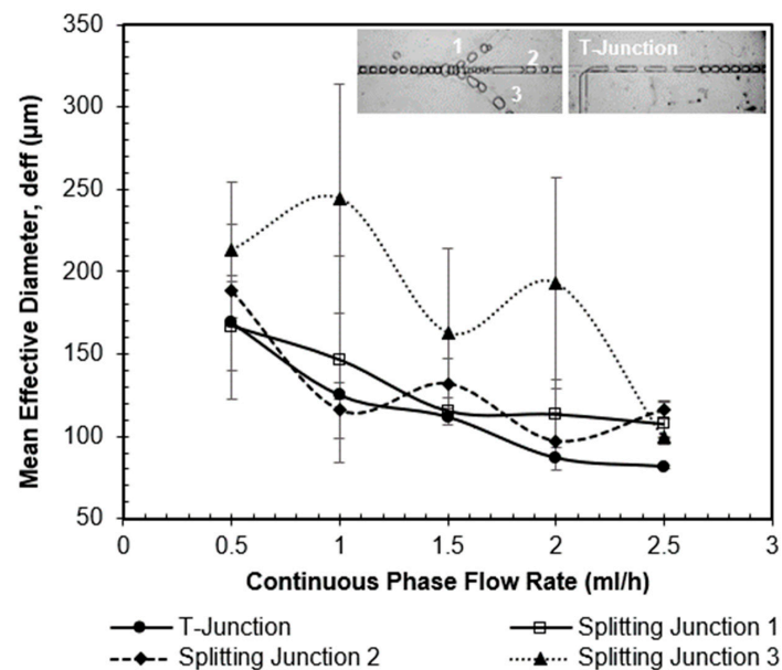
Figure 9. Average droplet size distribution with respect to different Q_c ranging from 0.5 to 2.5 mL/h in symmetrical bifurcating junction. Image indicates the region of interest for the droplet measurement. Error bars indicate the standard deviation in effective droplet size measurement of 30 droplets under fixed experimental condition.
