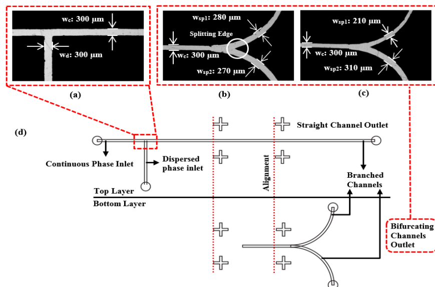
Figure 1. Images of xurographic positive-tone microchannel: (a) T-junction and bifurcated junction with (b) even (1:1) and (c) uneven aspect ratio (2:3) (where w_d denotes as the dispersed phase channel, w_c denotes as continuous phase channel, w_{sp1} denotes as first splitting junction and w_{sp2} denotes as second splitting junction, respectively). The sample images were taken using optical microscope using 2\times magnification. (d) Design of the microchannels composed of T-shaped and bifurcating channels using CorelDraw Graphics Suites X7. The red dotted line denotes the alignment profile of the bilayer microchannels.
