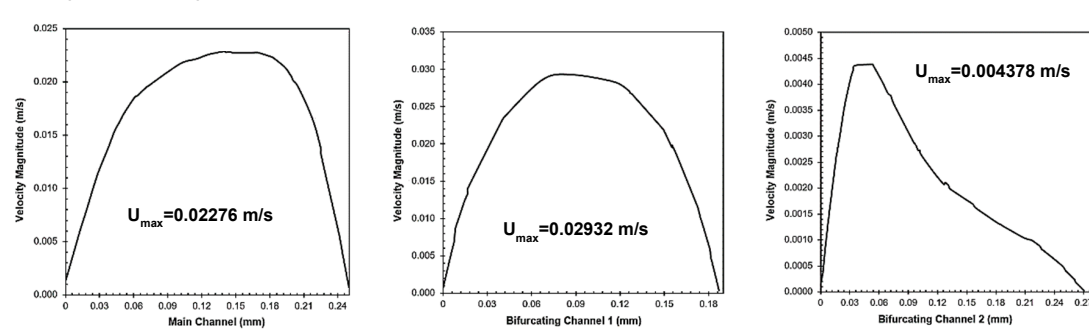
Figure 7. The simulated profile of velocity magnitude distribution along the direction of the continuous phase flow at the top layer of extended T-junction (for system: Q_c = 2 mL/h). The numbers indicate locations at which image profiles were taken.
