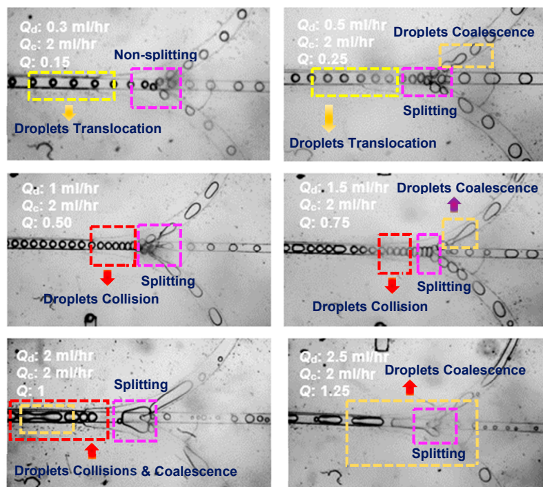
Figure 13. Droplet collision and coalescence phenomena in symmetrical splitting junctions at different flow rate ratio ( 0.15 < Q < 1.25 ) by fixing the Q_c and varying the Q_d .
