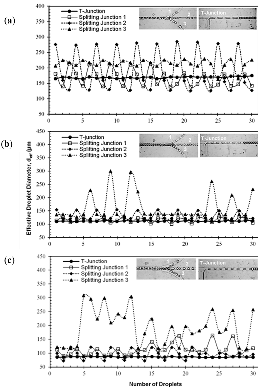
Figure 11. Droplet size distribution in different region of interests at Q_c of (a) 0.5 mL/h; (b) 1.5 mL/h; and (c) 2.0 mL/h, respectively. The images were taken under the optical microscope using high speed camera.
