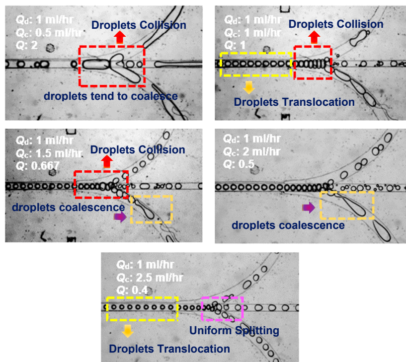
Figure 10. Droplet collision and coalescence phenomena in symmetrical splitting junctions at different flow rate ratio ( 0.4 < Q < 2 ) by fixing the Q_d and varying the Q_c .
