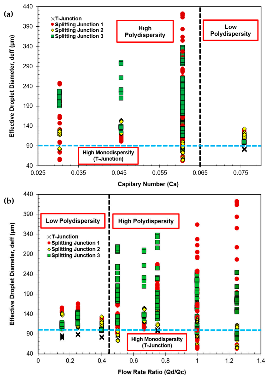
Figure 14. Distribution of droplet size in various regions of interest with respect to: (a) Capillary number and (b) flow rate ratio at symmetrical bifurcating junction.
