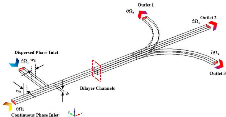
Figure 2. Schematic diagram of double planar microchannel. The droplets are subject to the 3D splitting point at the microchannel downstream where the mother droplets undergo fission and distributed into the trifurcation channels.
