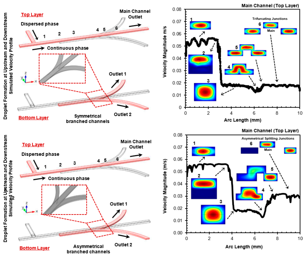
Figure 6. Evolution of flow profile at the upstream T-junction and downstream of symmetrical and asymmetrical splitting junctions (for system: Q_c = 2 mL/h).
