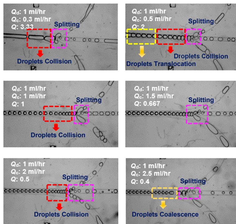
Figure 16. Droplet collision and coalescence phenomena in asymmetrical splitting junctions at different flow rate ratio ( 0.4 < Q < 3.33 ) by fixing the Q_d and varying the Q_c .
