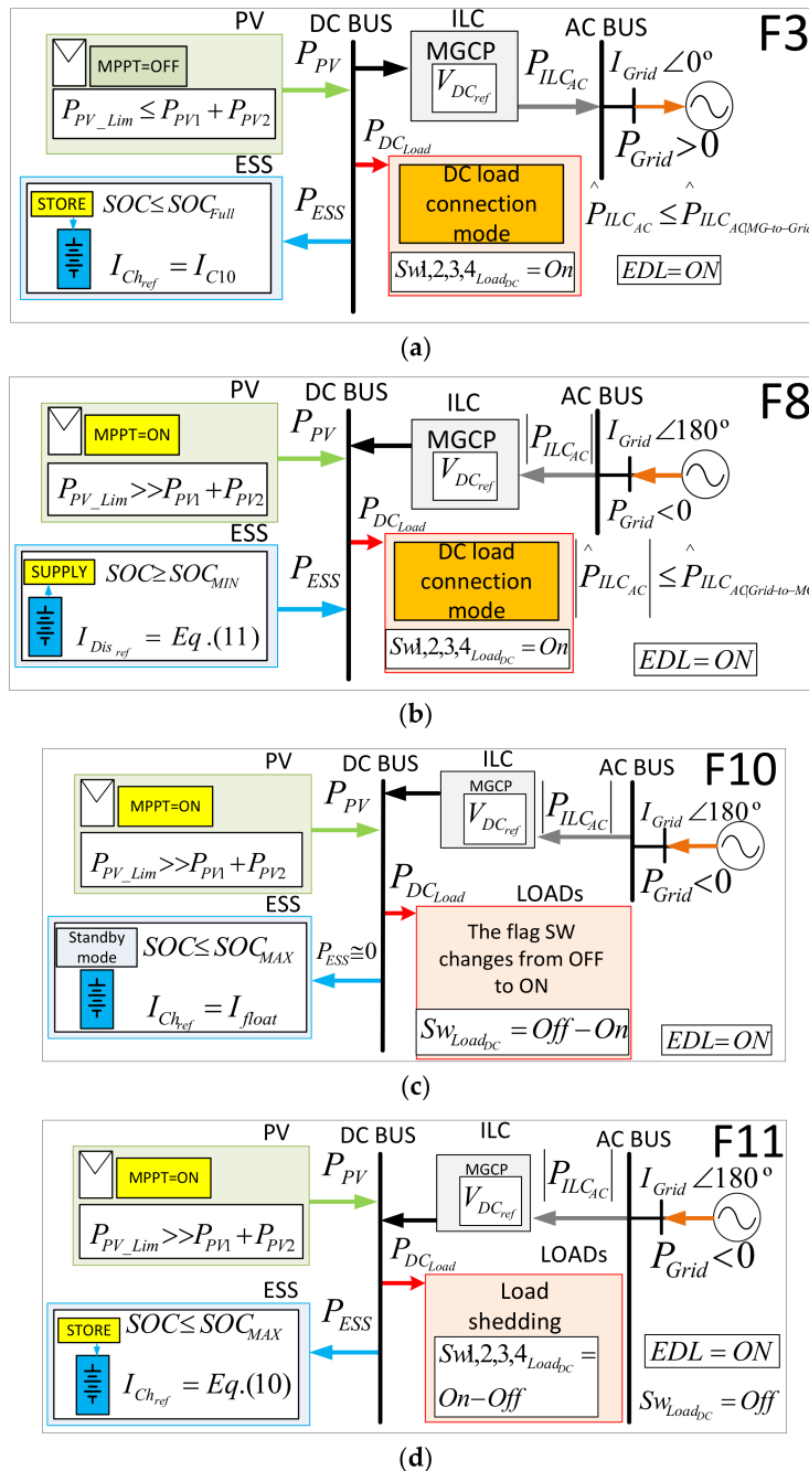
Figure 3. Power dispatch inside the MG after applying the operation functions: (a) F3; (b) F8; (c) F10 and (d) F11.
