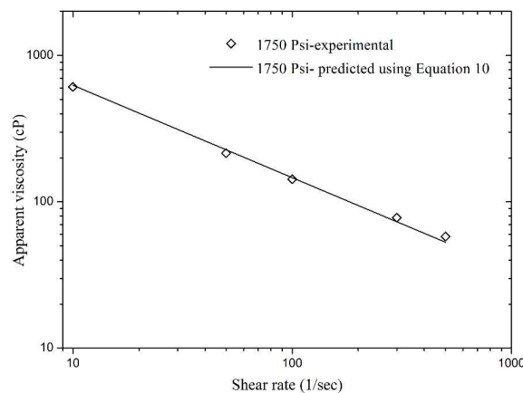
Figure 9. Validation of Equation (10).
