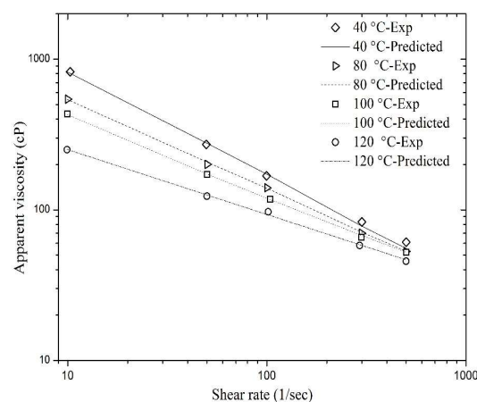
Figure 10. Match of the predicted viscosity values of s\text{CO}_2 foam using Equation (11) with the experimental data shown in Figure 2.
