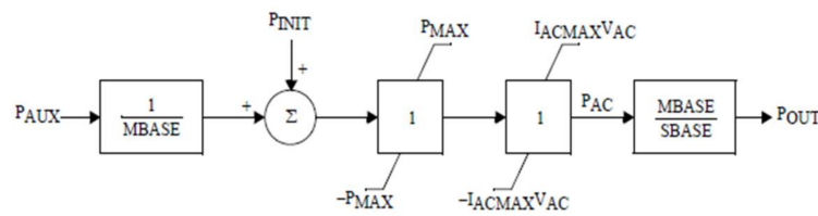
Figure 4. Diagram of CBEST BESS model from PSS/E [28].
