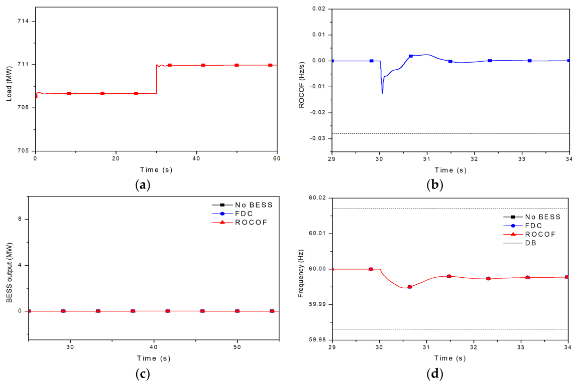
Figure 5. Power system load is increased by 2 MW: (a) Power system load; (b) Rate of Change of Frequency (ROCOF); (c) BESS output; (d) Power system frequency.
