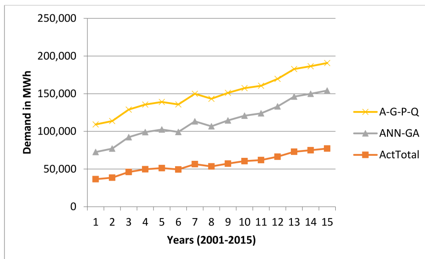
Figure 6. Comparison of ANN-G-P & A-G-P-Q.
