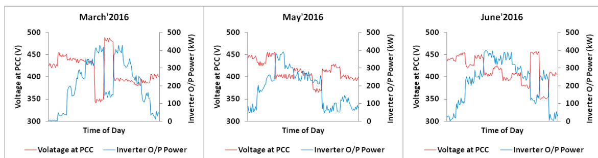
Figure 10. Inverter output power and voltage at the point of common coupling (PCC).
