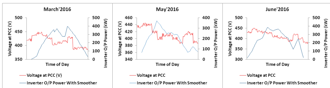
Figure 13. Inverter output power and voltage at PCC after introduction of the solar smoother.
