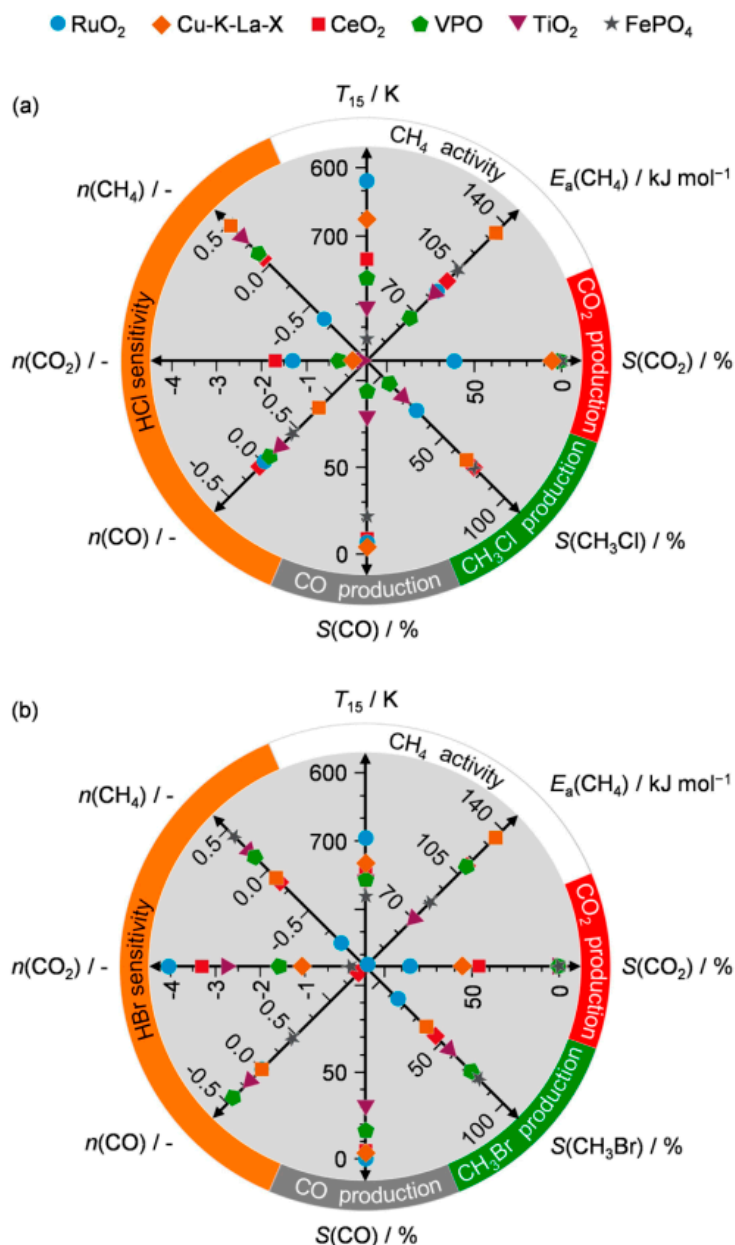
Figure 3. Overview of the catalytic descriptors in (a) methane oxychlorination and (b) methane oxybromination. The upper half of the radar charts classifies a material as a good oxyhalogenation catalyst if it combines high activity and low propensity to CO 2 formation. The bottom half classifies materials for their ability to produce CH 3 X. Reprinted from [61].
