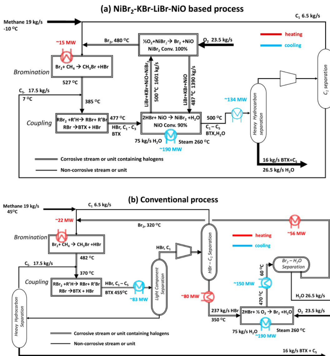
Figure 7. The proposed and conventional process for the conversion of methane to higher hydrocarbons [18].
