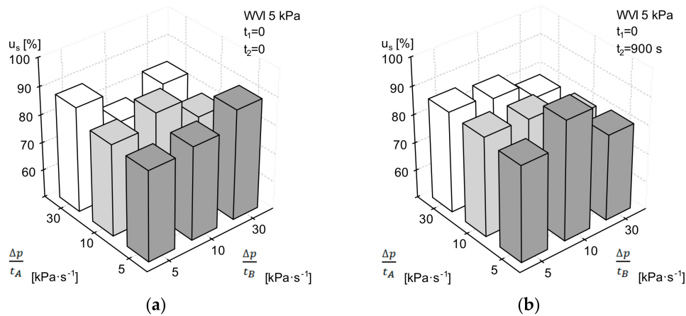
Figure 5. Dependence of the percentage of apple tissue staining u_s on the pressure change rate in the wet vacuum impregnation (WVI) cycle, for t_1 = 0 s and different values of t_2 : (a) t_2 = 0 s, (b) t_2 = 900 s.
