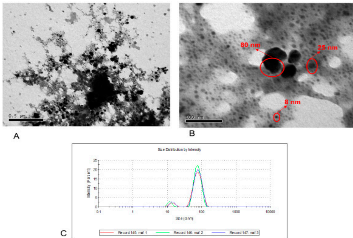
Figure 4. TEM images of Ns-AgNPs scale bar correspond to 0.5 \mu\text{m} (A) 100 nm (B) particle size distribution by DLS (C).
