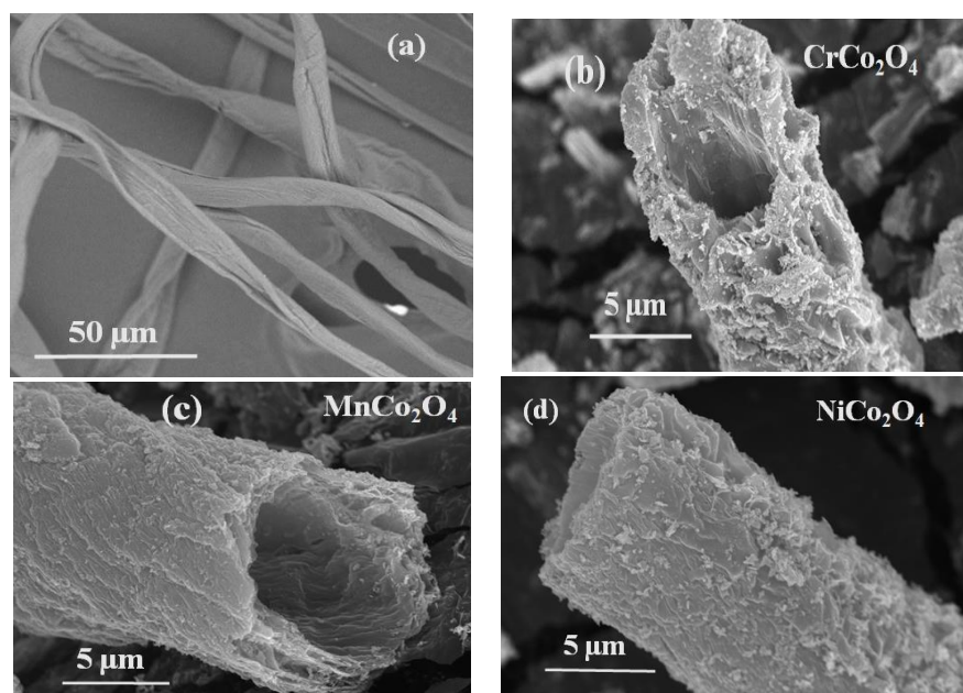
Figure 2. SEM images of (a) cotton fiber, (b), (c), and (d) bio-templated tubular \text{MCo}_2\text{O}_4 (M = Cr, Mn, Ni) structures.
