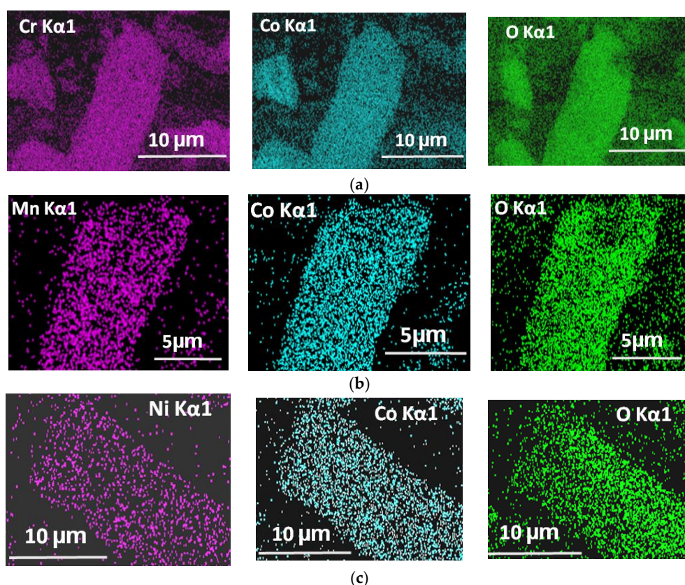
Figure 3. (a), (b), and (c) shows EDX mapping of tubular M\text{Co}_2\text{O}_4 ( M = \text{Cr}, \text{Mn}, \text{Ni} ) structures, respectively.
