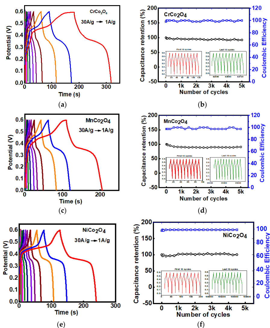
Figure 6. (a,c,e) show charge-discharge (CD) curves of tubular M\text{Co}_2\text{O}_4 ( M = \text{Cr}, \text{Mn}, \text{Ni} ) electrode measured in the current density window of 1 to 30 A/g in 3M KOH electrolyte, where red color CD curve is for 1A/g, blue color CD curve is for 1.5A/g, orange color CD curve is for 2A/g and continuously time is decreasing with increasing current density. (b,d,f) show cyclic stability (black color) and coulombic efficiency (blue color) tested at 10 A/g current density for 5000 cycles in 3M KOH electrolytes of M\text{Co}_2\text{O}_4 ( M = \text{Cr}, \text{Mn}, \text{Ni} ).
