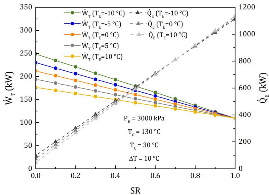
Figure 9. \dot{W}_T and \dot{Q}_E as a function of SR for Model III for different evaporator temperatures.
