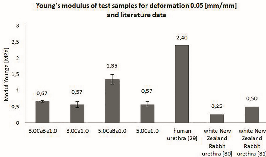
Figure 4. Young's modulus values for tubular alginate samples obtained in mechanical testing.
