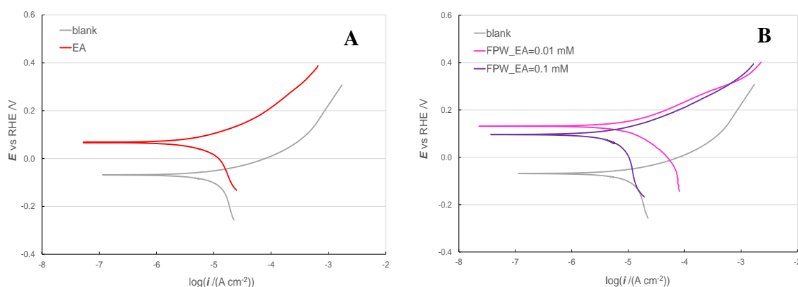
Figure 4. Potentiodynamic polarization curves (scan rate 0.5 \text{ mV s}^{-1} ) of Armco ® iron electrodes in aerated 0.05 M NaCl with 1 vol% methanol (grey lines). (A): with the addition of 10 \mu\text{M} ellagic acid (red line); (B): with different concentrations of FPW extract. Electrolyte temperature: 30 ^{\circ}\text{C} .
