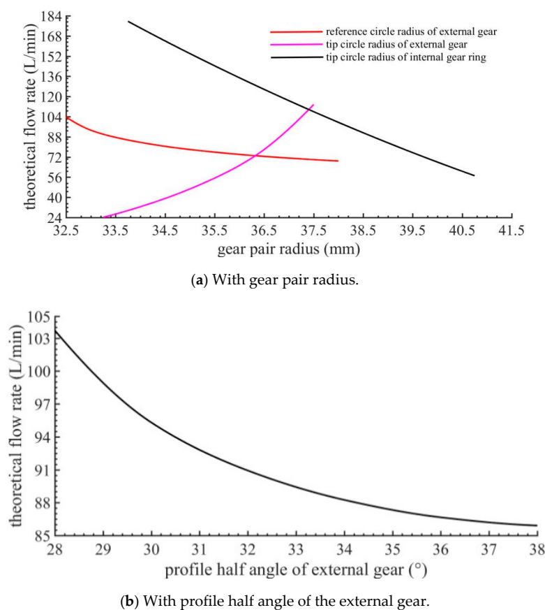
Figure 7. Change laws of the theoretical flow rate.
