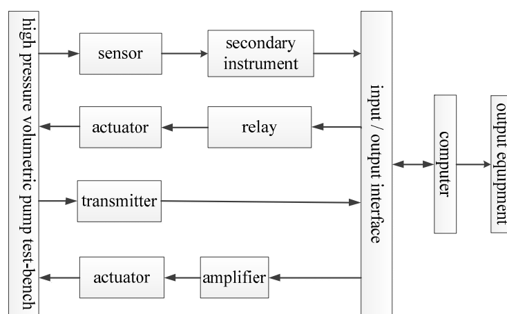
Figure 16. Overall design principle of test system.
