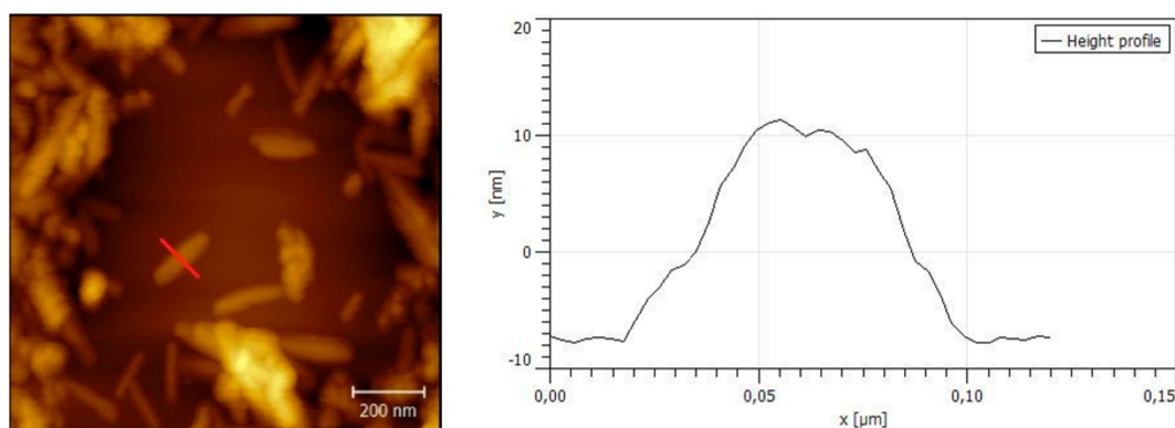
Figure 1. Atomic force microscopy image of graphene oxide (GO) captured on mica substrate together with height profile along the red line of interest on GO particle where the height is about 17 nm and lateral dimension about 200 nm in length.
