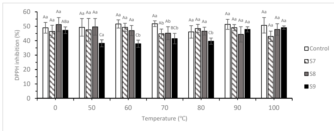
Figure 2. 2,2-diphenyl-1-picrylhydrazyl free radical (DPPH) free radical scavenging activities of MECs after water bath at different temperatures. MECs were reconstituted by methanol to achieve the 50-ppm curcumin concentration. All values are means of triplicates. Means followed by capital letters are significantly different due to thermal treatments ( p < 0.05 ). Means with different lowercase letters within the same set temperature group are significantly different caused by samples ( p < 0.05 ).
