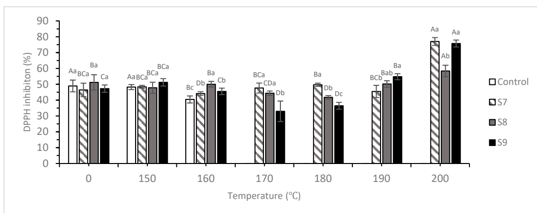
Figure 3. DPPH free radical scavenging activities of MECs after oven heating at different temperatures. MECs were reconstituted by methanol to achieve the 50-ppm curcumin concentration. All values are means of triplicates. Means followed by capital letters are significantly different due to thermal treatments ( p < 0.05 ). Means with different lowercase letters within the same set temperature group are significantly different caused by samples ( p < 0.05 ).
