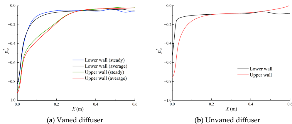
Figure 12. Time-averaged wall-pressure distributions.
