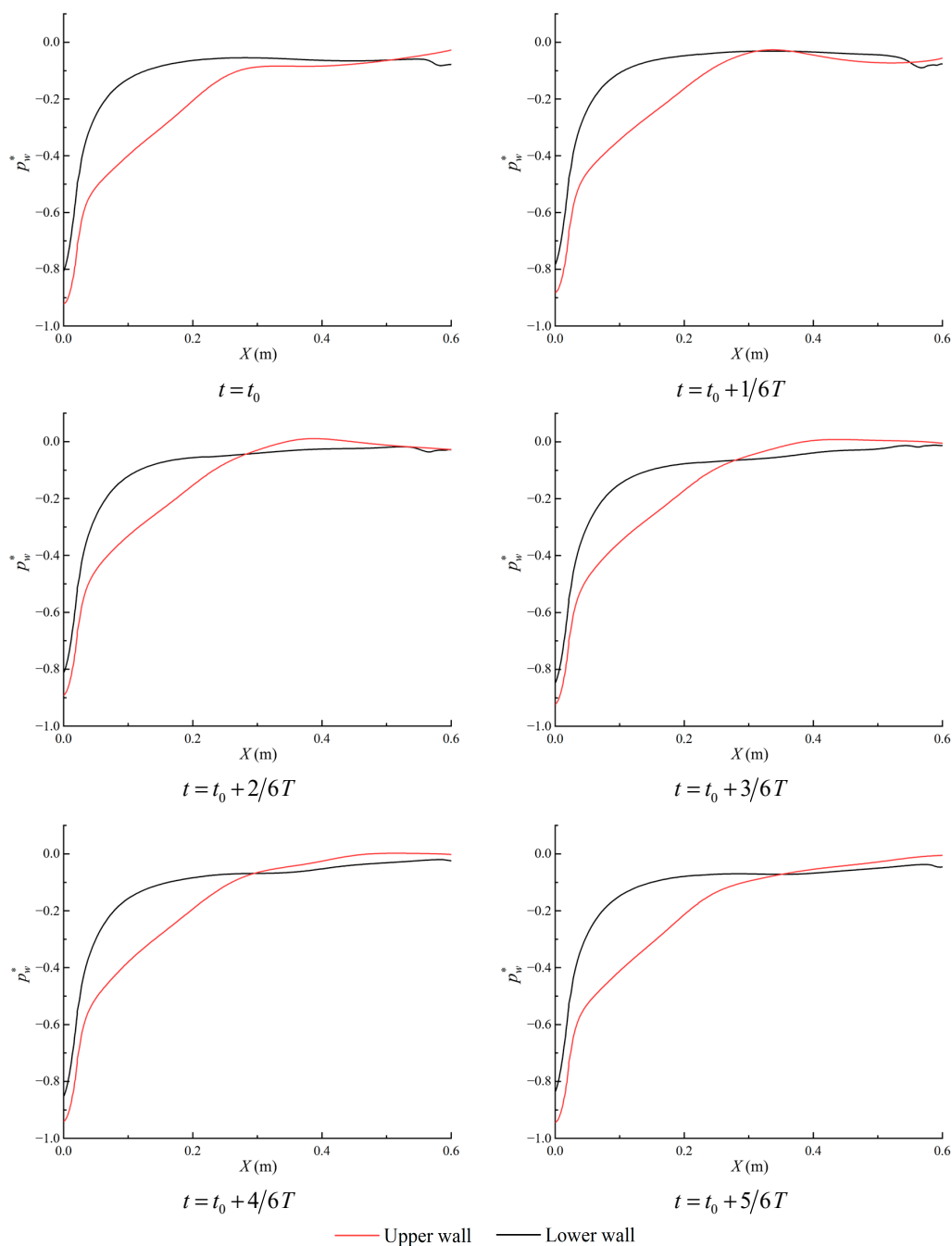
Figure 11. Distributions of wall pressure along diverging walls of the vaned diffuser.
