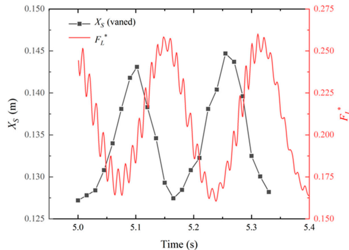
Figure 14. Lift force acting on a splitter vane.
