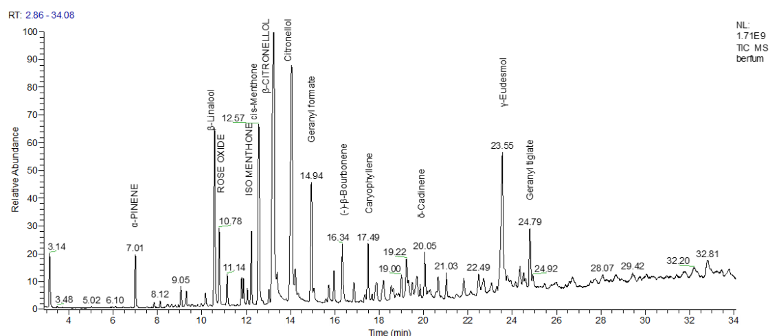
Figure 1. Total ion chromatogram of P. graveolens essential oil using GC–MS.
