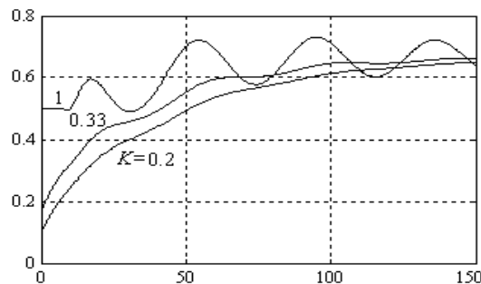
Figure 23. Control responses u(t) to a unit step reference for K = 0.2; 0.33; 1 .
