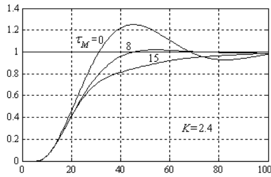
Figure 13. Responses y(t) to a unit step reference for K_M = 1.5 , T_{sM} = 73 and \tau_M = 0; 8; 15 .
