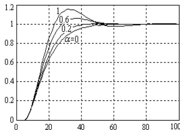
Figure 5. Responses y(t) to a unit step reference for process (31), G_M(s) = G_P(s) , K = 2 , and \alpha = 0; 0.2; 0.6; 1 .
