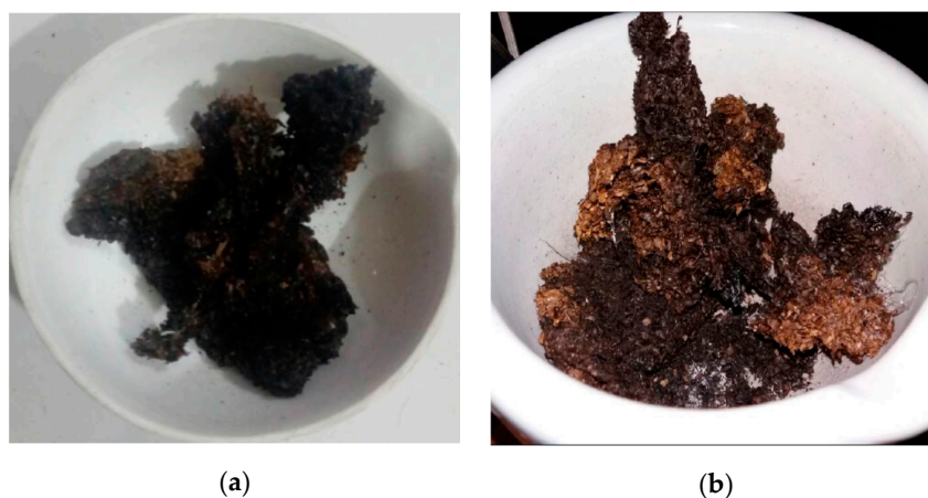
Figure 6. Flock of biomass particles in melting PP in co-pyrolysis with feed containing 50% weight of PP (a) and 75% weight of PP (b). Samples were taken when co-pyrolysis achieved 300 °C.
