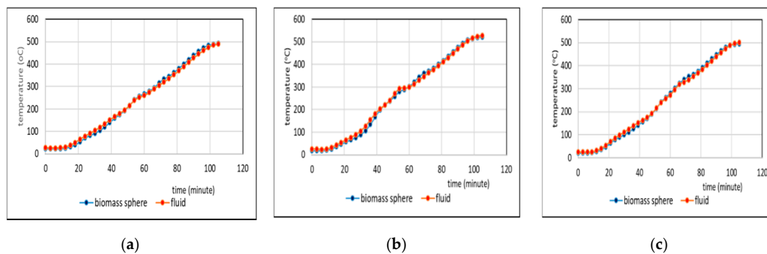
Figure 3. Comparison of temperatures of biomass spheres and biomass pyrolysis fluid taken at thermocouple #3 (a), thermocouple #4 (b), thermocouple #5 (c).
