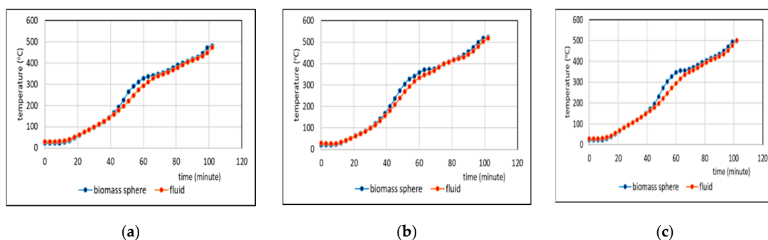
Figure 4. Comparison of temperatures of biomass spheres and co-pyrolysis fluid taken at thermocouple #3 (a), thermocouple #4 (b), thermocouple #5 (c). Co-pyrolysis used a feed containing 25% weight of PP.
