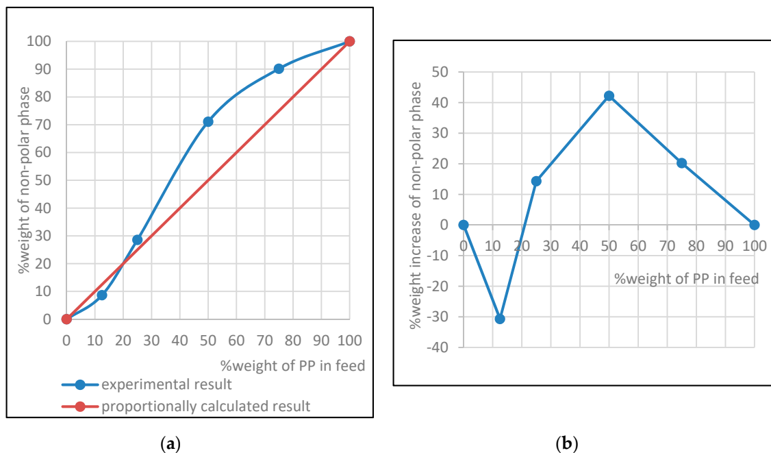
Figure 2. Experimental and theoretical fraction of non-oxygenated phase in bio-oil (a), the increase of non-polar fraction obtained experimentally compared to that obtained theoretically (b).
