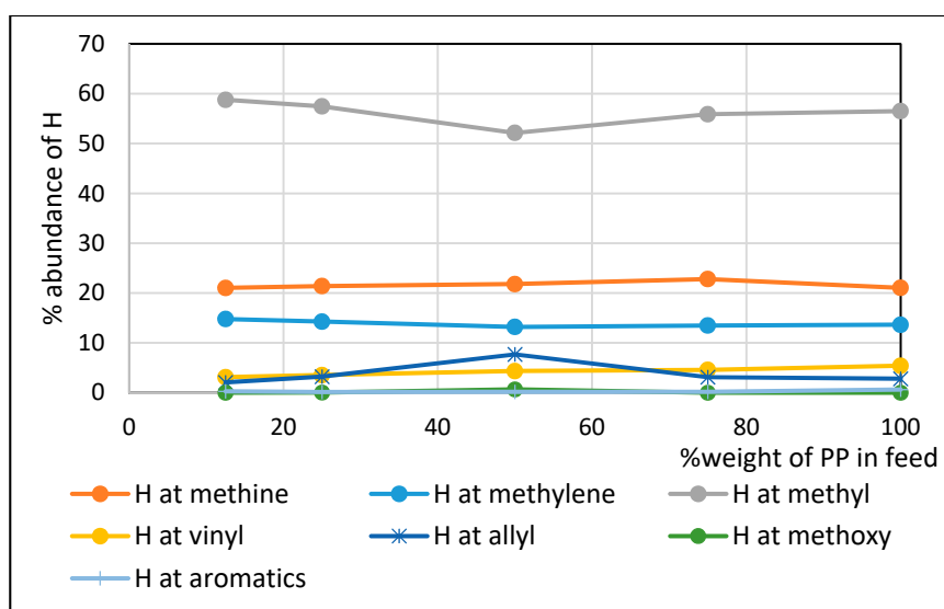
Figure 12. H-NMR analysis of wax.
