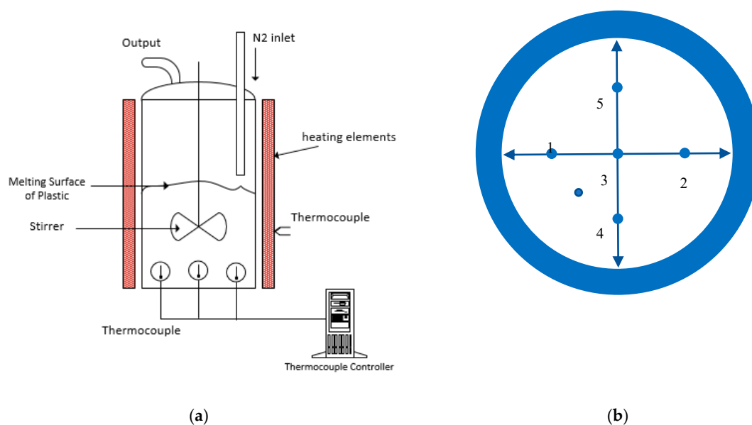
Figure 1. Inner schematics of the co-pyrolysis reactor (a), thermocouple configuration at the base of reactor (b).
