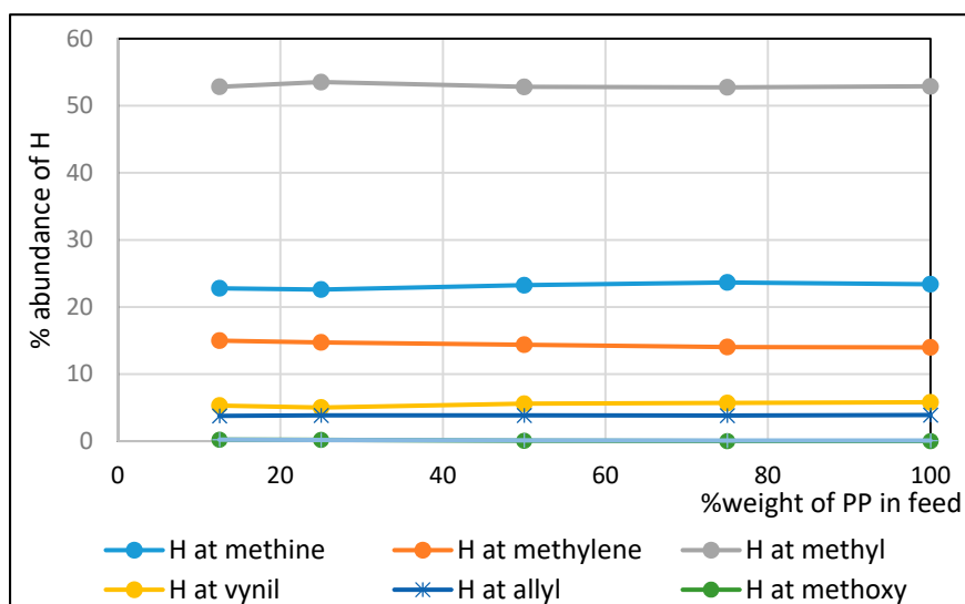
Figure 11. Effect of % weight of PP in feed mixture on %amount of H in non-polar fraction of bio-oil.
