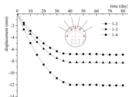
Figure 12. Monitoring results of roadway convergence. Red numbers 1–5 represent convergence monitor spots.
