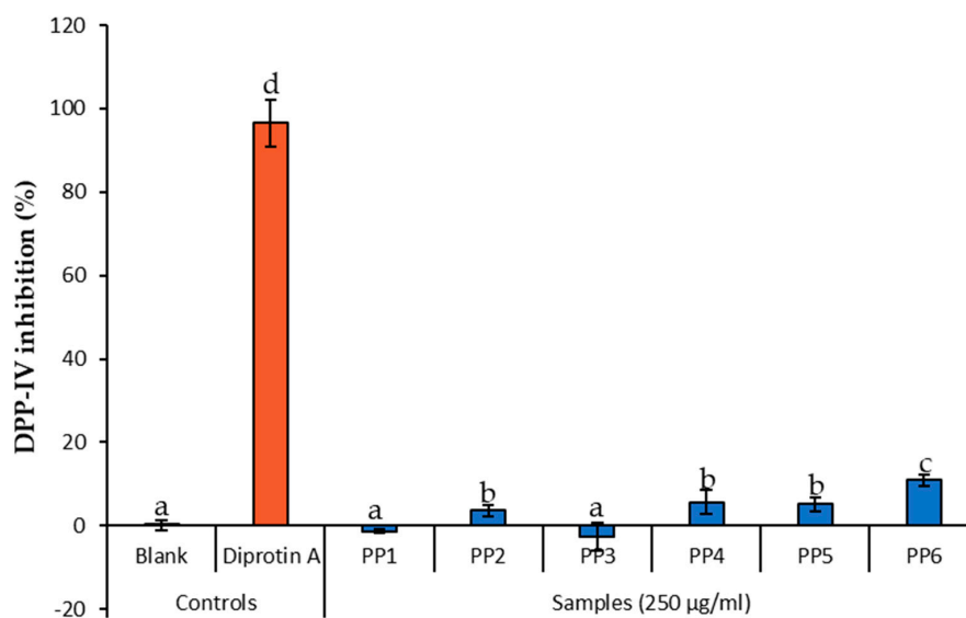
Figure 3. The inhibition of dipeptidyl peptidase-IV enzyme by different fractions from the methanolic extract of L. tetragona . The values are expressed as mean \pm SD (n = 5). Bars with different letters are significantly different ( p < 0.05 ).
