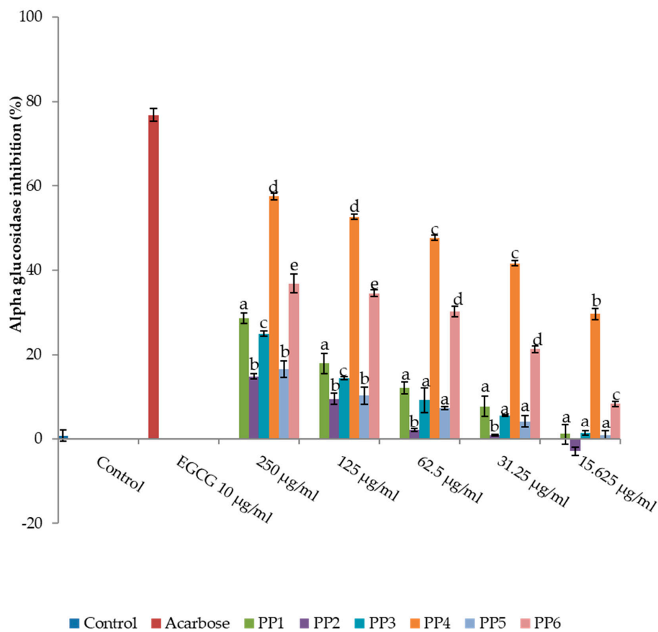
Figure 2. The inhibition of \alpha -glucosidase by different fractions from the methanolic extract of L. tetragona . The values are expressed as mean \pm SD (n = 5). Bars with different letters at each concentration are significantly different ( p < 0.05 ). EGCG = epigallocatechin gallate.
