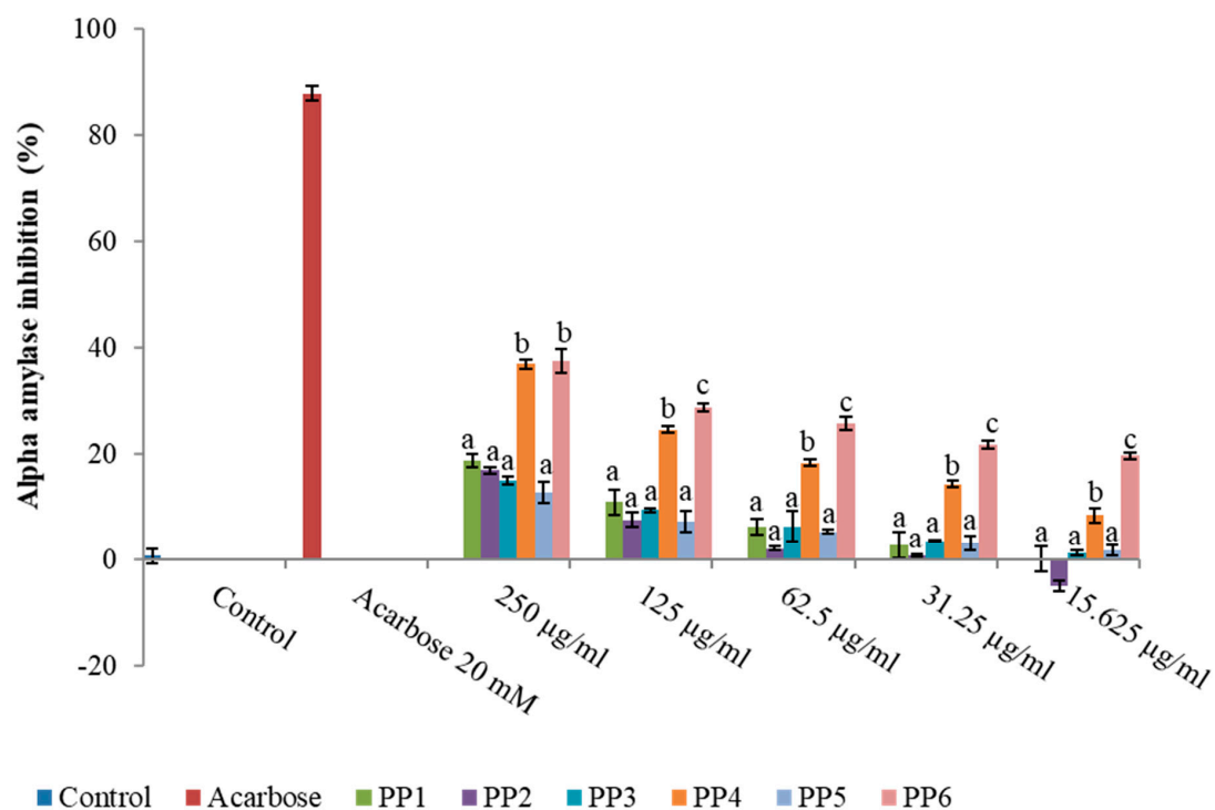
Figure 1. The inhibition of \alpha -amylase by different fractions from the methanolic extract of Lauridia tetragona . The values are expressed as mean \pm SD (n = 5). Bars with different letters at each concentration are significantly different ( p < 0.05 ).
