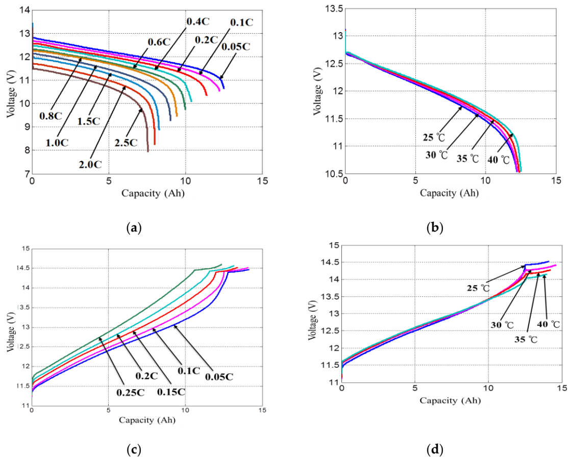
Figure 8. Experimental results of capacity measurement at: (a) various discharging currents at 25 °C; (b) 0.1C discharging current with various temperatures; (c) various charging currents at 25 °C; (d) 0.1C charging current with various temperatures.
