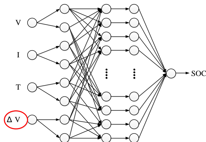
Figure 3. System configuration of the proposed adaptive network-based fuzzy inference system (ANFIS).
