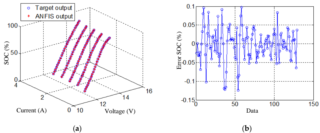
Figure 13. ANFIS SOC estimation results during charging at 25 °C: (a) results; (b) error.
