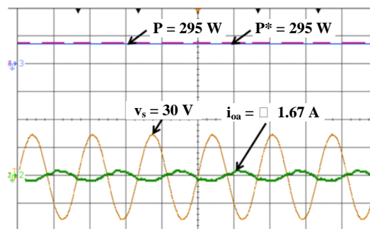
Figure 26. The inverter active power, voltage and current waveforms (phase-a) on the grid side corresponding to a 3A discharging current. ( t: 10 \text{ ms/div} ).
