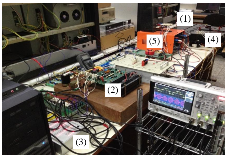
Figure 22. Photo of the experimental hardware implementation.
