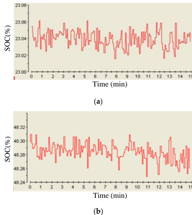
Figure 25. SOC estimated by ANFIS algorithm at discharging current of 3 A and voltages of (a) 11.5 V; (b) 11.9 V.
