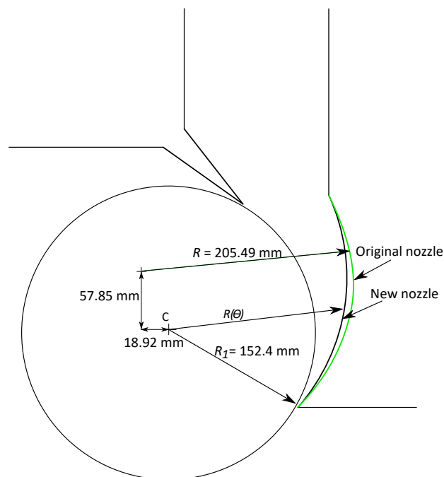
Figure 9. The original and new nozzle design for the 0.53 kW turbine.
