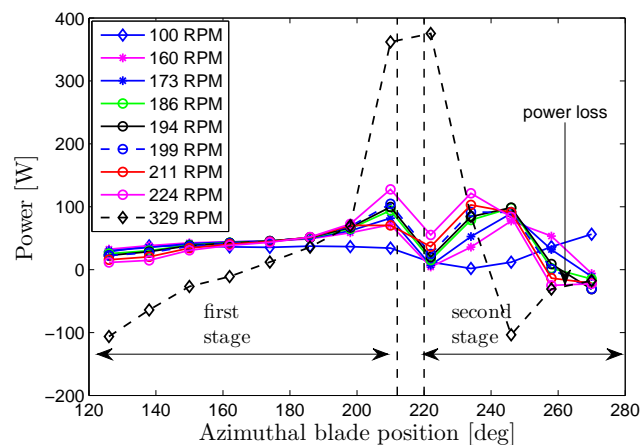
Figure 8. Azimuthal variation of power extraction per blade in the 0.53 kW turbine at \eta_{max} and \omega_{max} = 199.1 RPM ( Q = 46 lps and H = 1.337 m) [5].
