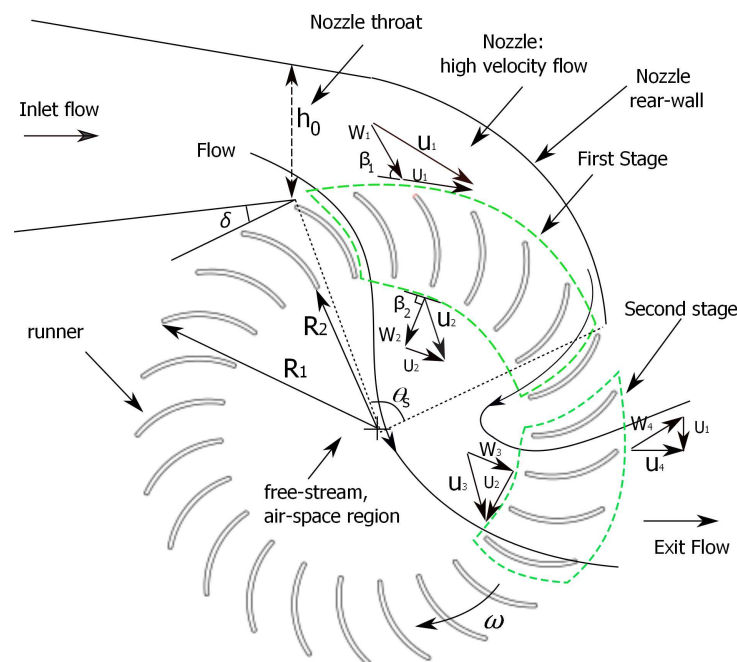
Figure 1. Schematic illustration of key geometrical parameters of crossflow turbine [2].
