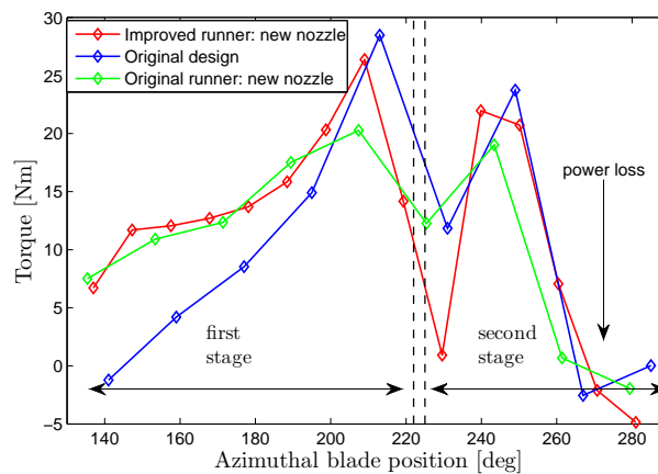
Figure 11. Comparison of torque production in the runner between the improved and the original runner with the new nozzle for the 7 kW turbine at \eta_{max} . Note that the original runner has N_b = 20 and \beta_{1b} = 30^\circ , whereas the new runner has N_b = 35 and \beta_{1b} = 39^\circ . For the purpose of comparison, the data are computed at each blade position and normalized with the torque for 35 blades. The first stage contributions for the original nozzle, the new nozzle with the original runner, and the new nozzle with improved runner are respectively 62%, 69%, and 73% [5].
