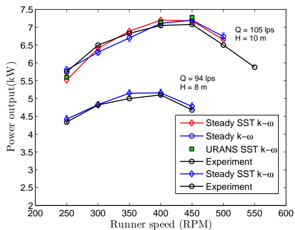
Figure 2. Comparison of CFD and experimental results for the power output of the 7 kW turbine at different flow rates and heads.
