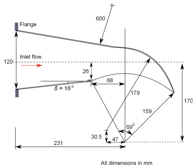
Figure 4. Schematic illustration of the 7 kW turbine [10] with \eta_{max} = 69\% . The three lines converge at the runner axis [5].
