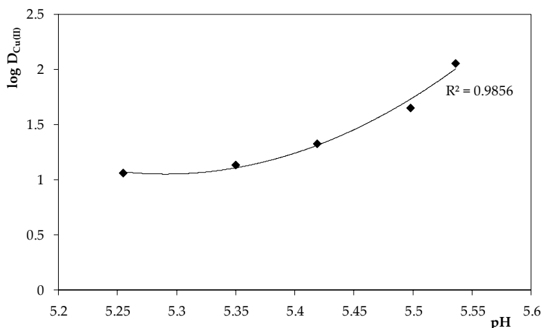
Figure 6. Relation \log D_{Cu(II)} = f(\text{pH}) in process of extraction Cu/(2,6-bis(4-methoxybenzoyl)-diaminopyridine) complexes.
