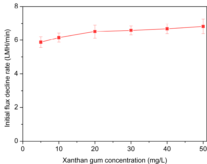
Figure 10. The initial fouling rate of xanthan gum at the presence of 1 mM \text{Ca}^{2+} .
