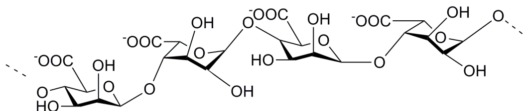
Figure 6. Chemical structure of alginate polysaccharide (GM blocks).
