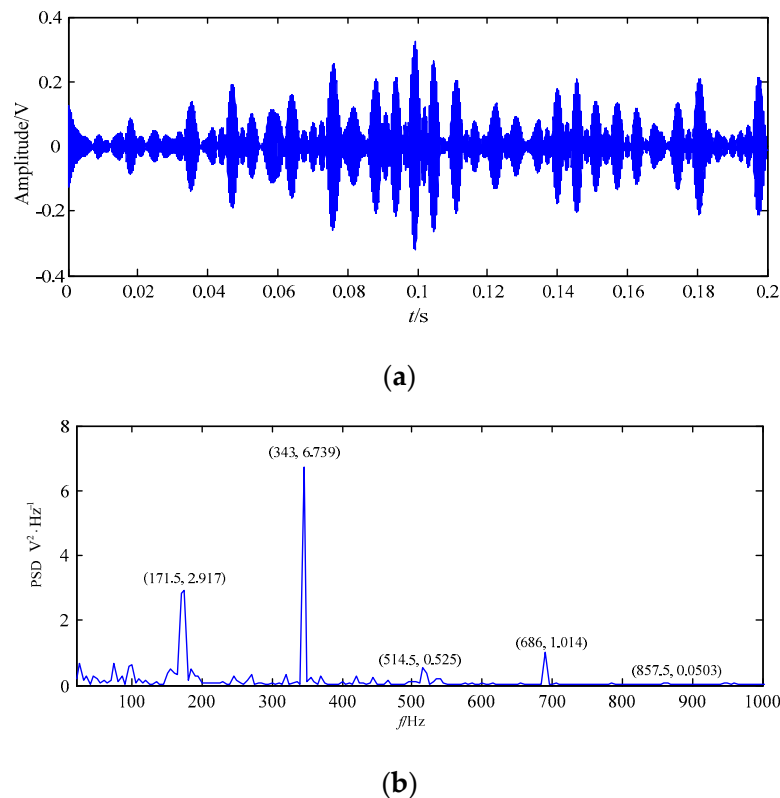
Figure 13. F_{13} got based on EWT. (a) Time domain wave; (b) power spectrum density.
