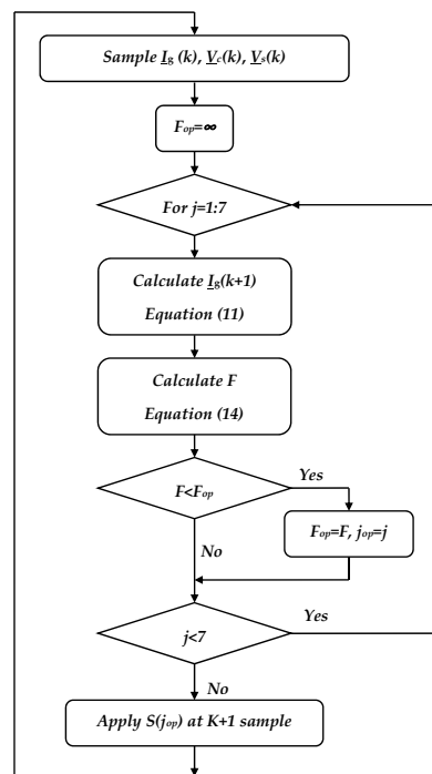
Figure 7. MPC algorithm flowchart.
