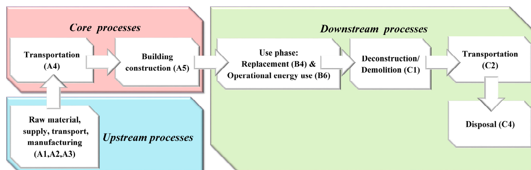
Figure 5. Life cycle processes and boundaries of the system.
